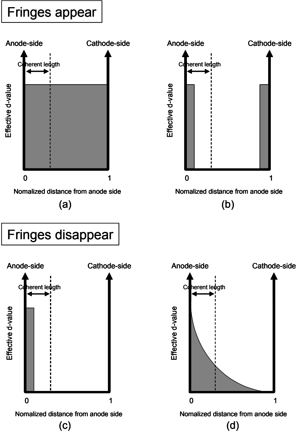
Figure 1.11 The d -value distribution determining the appearance of fringes in Maker-fringe pattern. Cases (a) and (b) lead to the oscillation in SH intensity, and cases (c) and (d) to the absence of fringe.
