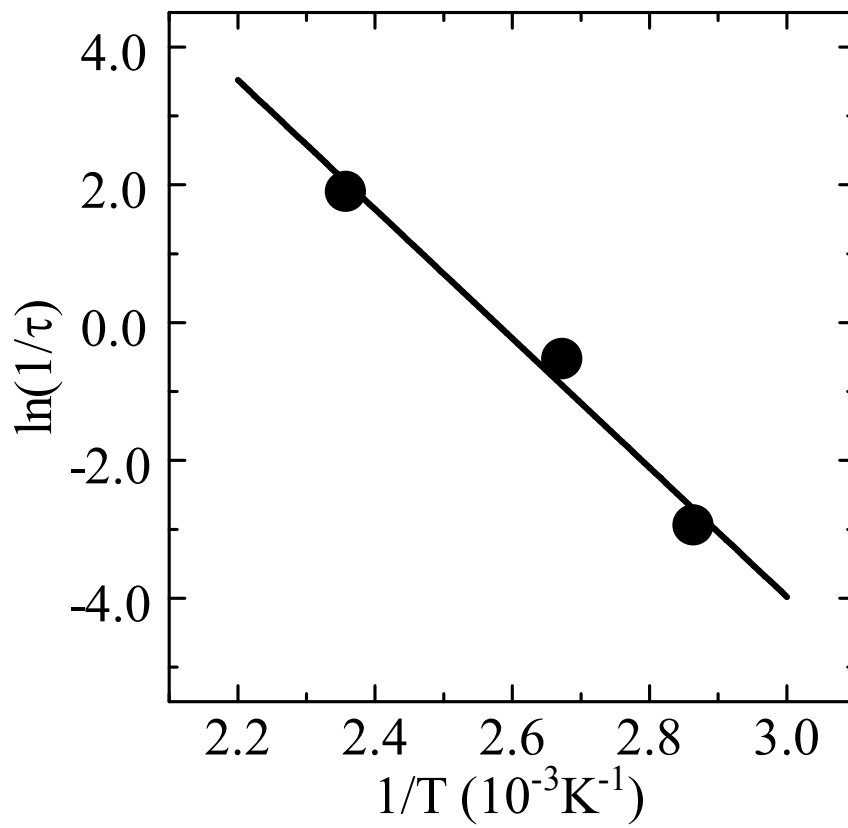
Figure 1.19 Temperature dependence of the relaxation time for observed SH intensity in 15\text{Nb}_2\text{O}_5 \cdot 85\text{TeO}_2 glass poled at 260^\circ\text{C} . The straight line is the Arrhenius straight line drawn by the least-squares method.
