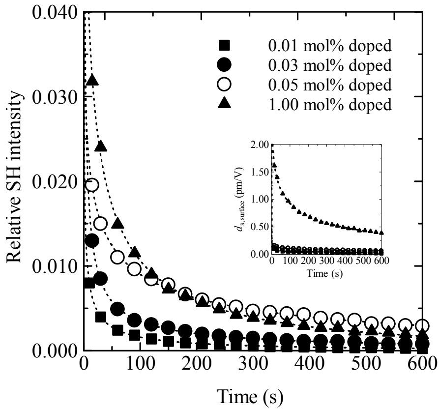
Figure 2.5 Time variation of SH intensity from the \text{V}_2\text{O}_5 -doped 15\text{Nb}_2\text{O}_5 \cdot 85\text{TeO}_2 glass samples after ceasing optical poling. Relative SH intensity to the maximum SH intensity in Y-cut \alpha -quartz is taken in the vertical. The inset is the effective d-value at the incidence surface which is calculated from the relative SH intensity.
