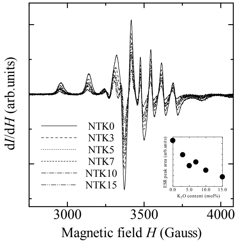
Figure 2.11 ESR spectra for \text{VO}^{2+} ion in \text{K}_2\text{O-Nb}_2\text{O}_5\text{-TeO}_2 glass doped with 0.5 mol% \text{V}_2\text{O}_5 . The inset shows ESR peak area derived from the spectra plotted against \text{K}_2\text{O} content.
