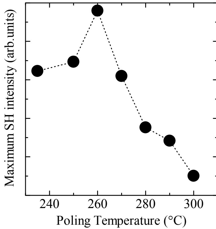
Figure 1.16 Poling temperature dependence of the maximum SH intensity generated in thermally/electrically poled 15\text{Nb}_2\text{O}_5\cdot 85\text{TeO}_2 glass.
