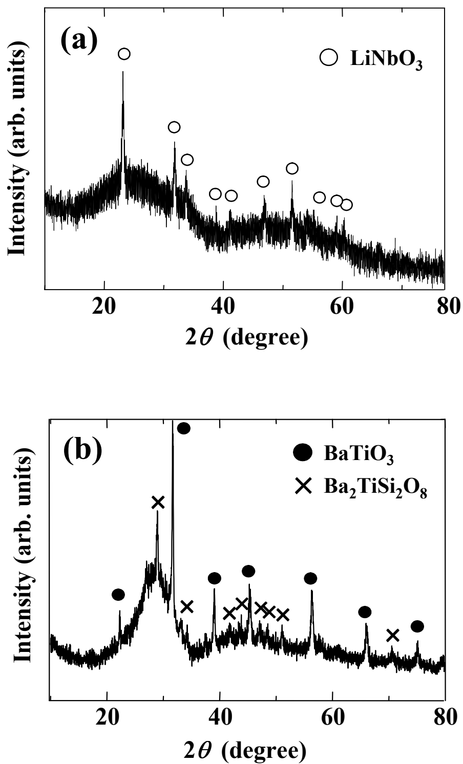
Figure 3.4 X-ray diffraction patterns for laser-induced precipitates (a) in 32.5\text{Li}_2\text{O}\cdot 27.5\text{Nb}_2\text{O}_5\cdot 40.0\text{SiO}_2 glass (sample 1) and (b) in 5.0\text{Na}_2\text{O}\cdot 36.0\text{BaO}\cdot 39.0\text{TiO}_2\cdot 20.0\text{SiO}_2 glass (sample 4).
