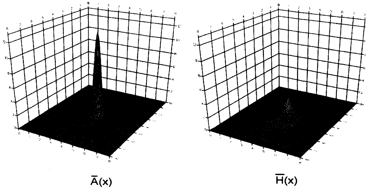
Figure 3: Pulse-like localized patterns for G-M in 2D ([4]).
