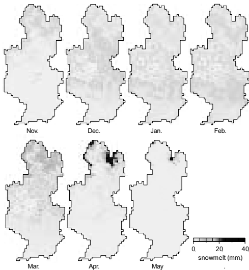
Fig. 13 Monthly snowmelt (1979-2000)
