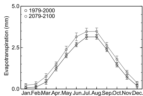
Fig. 10 Monthly evapotranspiration
