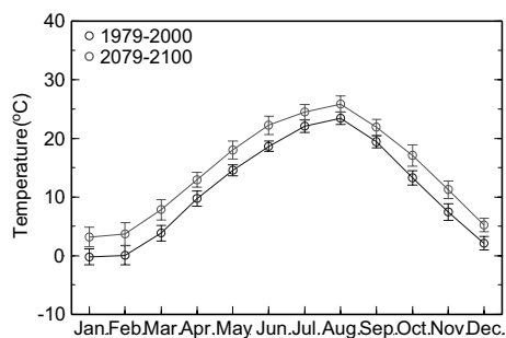
Fig. 9 modified temp.
