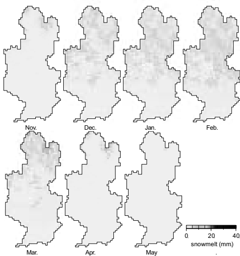
Fig. 14 Monthly snowmelt (1979-2000)
