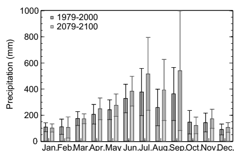
Fig. 8 modified precipitation
