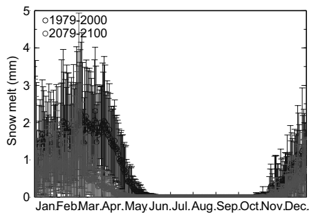
Fig. 12 Monthly snowmelt
