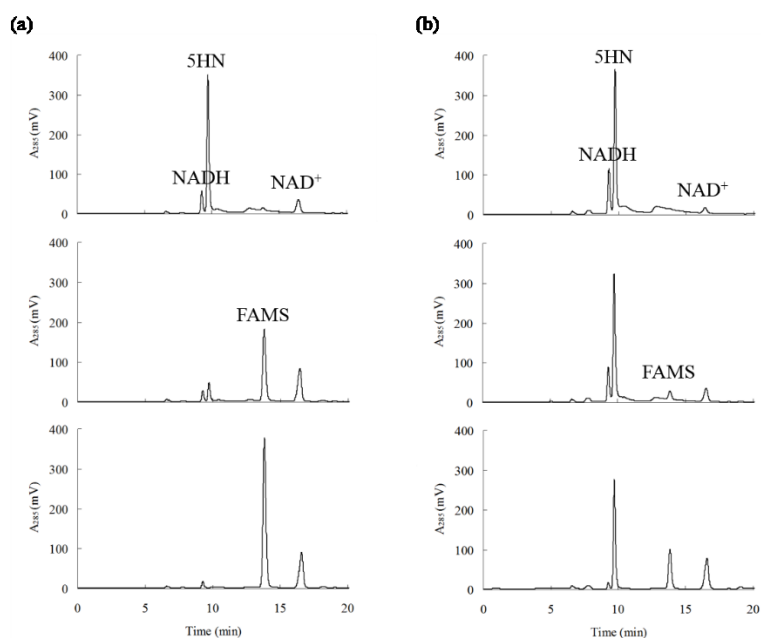
Figure 5. HPLC elution patterns of the substrates and products in the reaction mixtures with the WT enzyme and the Y270F mutant. (a) Reaction with the WT enzyme. (b) Reaction with the Y270F mutant. Elution patterns of the reaction mixtures stopped at 1, 5 and 30 min are shown in the top, middle and bottom panels, respectively.
