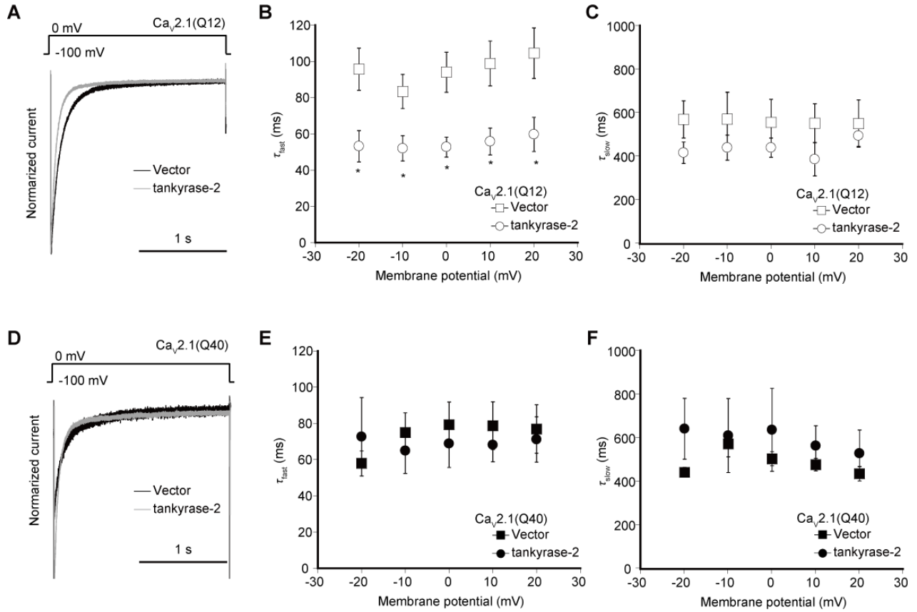
Fig. 6 Effects of tankyrase-2 on the inactivation kinetics of P/Q-type Ca v 2.1 channel with Q12 or Q40. (A, D) The peak amplitudes were normalized for Ba 2+ currents elicited by 2-s pulses to 0 mV from a holding potential ( V_h ) of −100 mV before and after expression of tankyrase-2. Ca v 2.1 with Q12 (A) or Q40 (D) was expressed in BHK cells. (B, C) Voltage dependence of the two inactivation time constants, \tau_{fast} (B) and \tau_{slow} (C) in polyQ12-expressing cells. The mean inactivation time constants were plotted as a function of test potential from −20 mV to 30 mV. * P < 0.05 compared with Vector control. (E, F) Voltage dependence of the two inactivation time constants, \tau_{fast} (E) and \tau_{slow} (F) in polyQ40-expressing cells. The mean inactivation time constants were plotted as a function of test potential from −20 mV to 30 mV. Data points are mean ± SEM.
