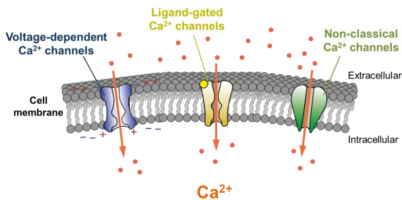
Fig. 1 Classes of \text{Ca}^{2+} -permeable ion channels.
