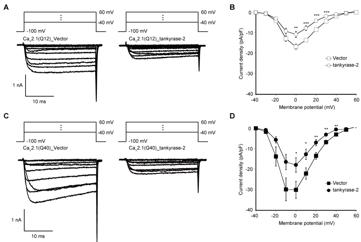
Fig. 3 Effects of tankyrase-2 on the current density-voltage ( I - V ) relationships of P/Q-type Ca v 2.1 with Q12 or Q40. (A, C) Representative traces of Ba 2+ currents with or without tankyrase-2 on application of test pulses from -40 to 60 mV with 10-mV increments from a V h of -100 mV. Ca v 2.1 with Q12 (A) or Q40 (C) was expressed in BHK cells. (B, D) I - V relationships of P/Q-type Ca v 2.1 with Q12 (B) or Q40 (D). * P < 0.05, ** P < 0.01, *** P < 0.001 compared with Vector control. Data points are mean ± SEM.
