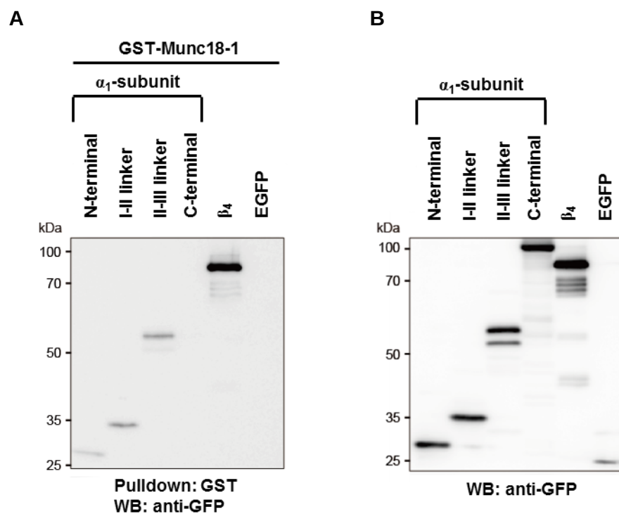
Fig. 2 Interaction of the VDCC \alpha_1 -subunit with Munc18-1. (A) GST fusion Munc18-1 immobilized on glutathione-Sepharose beads were incubated with cell lysates obtained from GFP tagged fragments of the \alpha_1 -subunit, full-length \beta_{4b} -subunit, and control GFP vector-transfected HEK293 cells. Bound proteins were analyzed by western blotting using an antibody for GFP. WB, western blotting. (B) Expression and input of EGFP-tagged fragments of the \alpha_1 -subunit, full-length \beta_{4b} -subunit were analyzed by western blotting.
