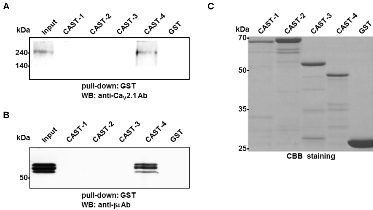
Fig. 3 Complex formation of CAST with VDCCs through the \beta_4 -subunit. (A, B) The GST fusion proteins containing various CAST regions (Fig. 1B) as well as GST alone were immobilized on glutathione-Sepharose beads. The detergent extract of the mouse brain synaptosomal fraction was then incubated with the beads, and proteins that bound to the beads were analyzed by western blotting using the indicated antibodies. The endogenous VDCC \alpha_1 -subunit (anti- \text{Ca}_v2.1 ) and VDCC \beta_4 -subunit were pulldowned by CAST-4. Ab, antibody; WB, western blotting. (C) Coomassie brilliant blue (CBB) staining of loaded GST fusion proteins.
