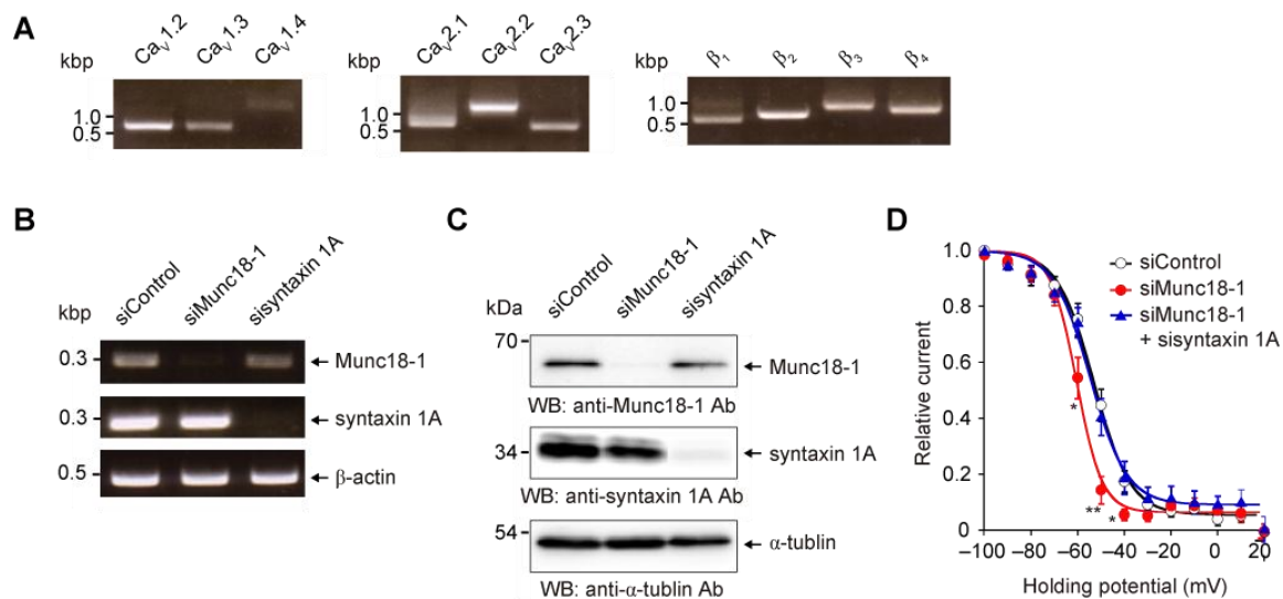
Fig. 6 Physiological relevance of Munc18-1 effects on VDCC function. (A) Molecular characterization of NG108-15 cells. RNA expression analysis of \alpha_1 - and \beta -subunits using RT-PCR in NG108-15 cells. (B) RT-PCR analysis of Munc18-1 and syntaxin 1A RNA expression in NG108-15 cells treated with GAPDH siRNA (siControl), Munc18-1 specific siRNA (siMunc18-1) and syntaxin 1A specific siRNA (sisyntaxin 1A). \beta -actin was used as loading control. (C) Western blotting analysis of Munc18-1 and syntaxin 1A protein expression in NG108-15 cells. \alpha -tubulin was used as loading control. Ab, antibody; WB, western blotting. (D) Effects of siRNA for Munc18-1 or Munc18-1 and syntaxin 1A on the inactivation curves for VDCCs in NG108-15 cells. Normalized test pulse currents were plotted against potentials of the 2-s V_h displacement and fitted to the single Boltzmann's equation. * P < 0.05 , ** P < 0.01 versus siControl. Data points are mean \pm SEM.
