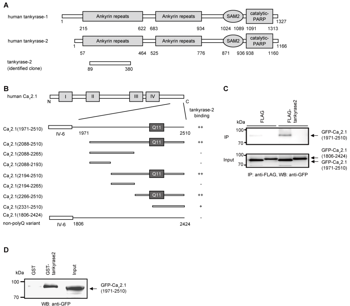
Fig. 1 Direct interaction of tankyrase-2 with the C-terminus of Ca_v2.1 subunit. (A) Domain structure of tankyrase-1 and tankyrase-2. Sterile alpha motif (SAM) 2 domain and catalytically active poly-ADP ribose polymerase (PARP) domain are located at the C-terminus of tankyrase. The protein region encoded by identified clone is also indicated. (B) Mapping of tankyrase-2 binding sites on the C-terminus of Ca_v2.1 subunit by the yeast two-hybrid assay. Ca_v2.1 subunit constructs in bait vectors were tested with tankyrase-2 in the prey vector. The interactions were scored by \beta -galactosidase activity and His^+ prototrophy. (C) Interaction of recombinant C-terminus of Ca_v2.1 and tankyrase-2 in HEK293 cells. The interaction was evaluated by immunoprecipitation with antibody for FLAG, followed by western blotting with antibody for GFP. Ca_v2.1 (1971-2510) or Ca_v2.1 (1806-2424) is a variant with or without polyQ domain, respectively. IP, immunoprecipitation; WB, western blotting. (D) Pulldown assay of C-terminus of Ca_v2.1 with GST fusion tankyrase-2. GST fusion proteins immobilized on glutathione-Sepharose beads were incubated with cell lysates obtained from GFP- Ca_v2.1 (1971-2510)-transfected HEK293 cells. Bound proteins were analyzed by western blotting using antibody for GFP.
