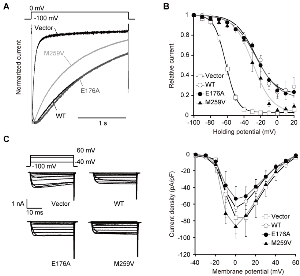
Fig. 5 Autism mutations affect RIM3 regulation of \text{Ca}_v2.2 VDCCs. (A) Effect of WT, E176A and M259V RIM3 on inactivation kinetics of N-type \text{Ca}_v2.2 VDCCs in HEK293 cells co-expressing \alpha_2/\delta and \beta_1 subunits. Peak amplitudes were normalized for \text{Ba}^{2+} currents elicited by 2-s pulses to 0 mV from a V_h of -100 mV, with or without WT, E176A, and M259V RIM3. (B) Effect of WT, E176A, and M259V on inactivation curves of N-type \text{Ca}_v2.2 currents. Voltage dependence of inactivation determined by measuring peak current amplitudes evoked by 20-ms test pulses to 5 mV following 2-s prepulses to potentials from -100 to 20 mV in 10-mV increments from a V_h of -100 mV, were fitted using Boltzmann's equation. (C) Effect of WT, E176A, and M259V on \text{Ca}_v2.2 current amplitudes. Left , representative traces in HEK293 cells co-expressing \alpha_2/\delta and \beta_1 subunits for \text{Ba}^{2+} currents evoked by test pulses from -40 to 60 mV in 10-mV increments. Right , current density-voltage relationship of \text{Ca}_v2.2 with V_h of -100 mV. Data points are mean \pm SEM.
