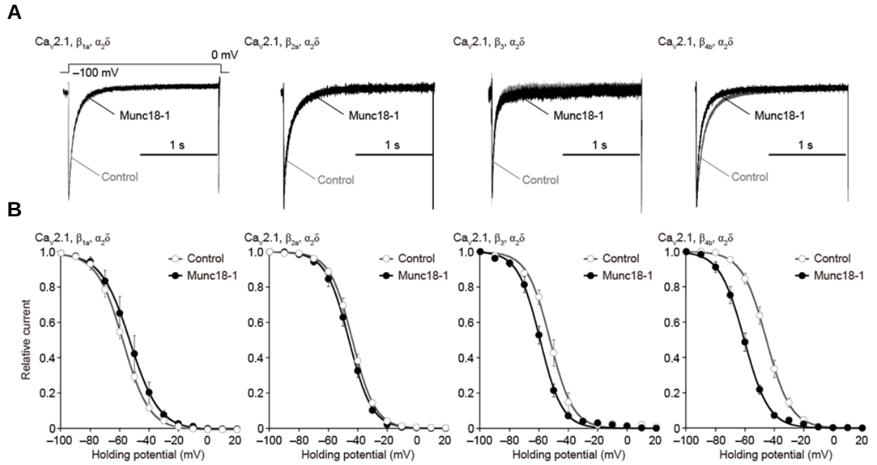
Fig. 3 Effects of Munc18-1 on the inactivation properties of recombinant P/Q-type VDCC currents.
