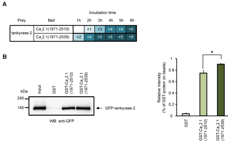
Fig. 2 The interaction between C-terminus of Ca v 2.1 and tankyrase-2 is augmented by elongated-polyQ. (A) Interaction of tankyrase-2 and C-terminus of Ca v 2.1 with different polyQ length by yeast two-hybrid assay. Two constructs in bait vectors were tested with tankyrase-2 in the prey vector. The interactions were scored by \beta -galactosidase activity. The blue color phenotype was scored (+5: very strong, +4: strong, +3: intermediate, +2: weak, +1: very weak, blank: no binding). (B) Pulldown assay of tankyrase-2 with GST fusion C-terminus proteins of Ca v 2.1. Left , representative images of western blotting. GST fusion proteins immobilized on glutathione-Sepharose beads were incubated with cell lysates obtained from GFP-tankyrase-2-transfected HEK293 cells. Bound proteins were analysed using antibody for GFP. WB, western blotting. Right , Quantitative analysis of western blotting. Relative intensities were quantified using NIH software and normalized by GST-fusion protein on beads. * P < 0.05 . Data points are mean \pm SEM.
