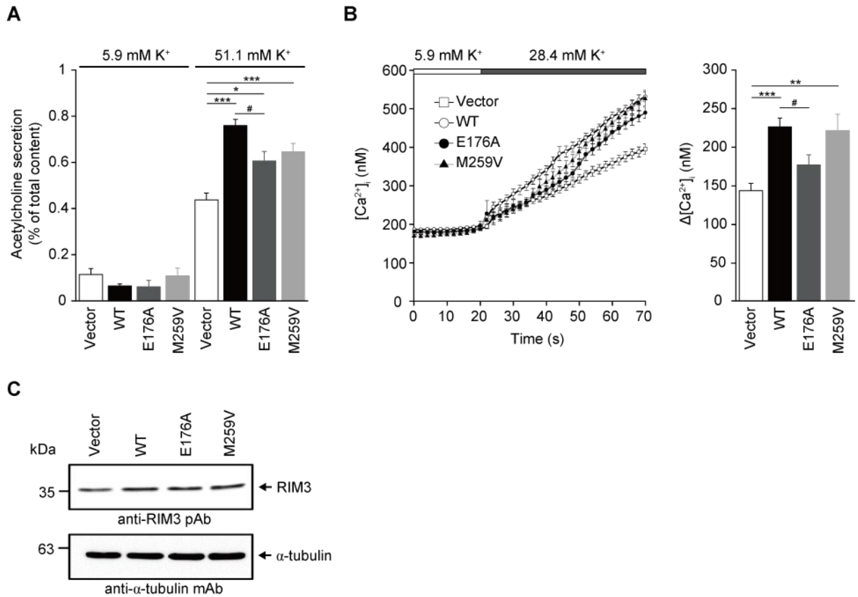
Fig. 6 Autism mutations affect RIM3 potentiation of ACh release. (A) Effect of WT, E176A and M259V RIM3 on depolarization-dependent ACh release from ChAT-cotransfected PC12 cells. Secreted ACh was determined as a percentage of cellular content for each dish. * P < 0.05 and *** P < 0.001 versus vector; # P < 0.05 versus WT. (B) Effect of WT, E176A, and M259V RIM3 on Ca 2+ response to elevation of extracellular K + concentration from 5.9 to 28.4 mM. Average time course (left) and [Ca 2+ ] i increase at 30 s after treatment with 28.4 mM K + solution (right). Numbers of PC12 cells analyzed were 75, 59, 51, and 42 for transfection of vector, WT, E176A, and M259V RIM3, respectively. ** P < 0.01 and *** P < 0.001 versus vector; # P < 0.05 versus WT. (C) Protein expression analysis of WT RIM3 and the mutants using western blotting in PC12 cells. α-tubulin was used as a loading control. Data points are mean ± SEM.
