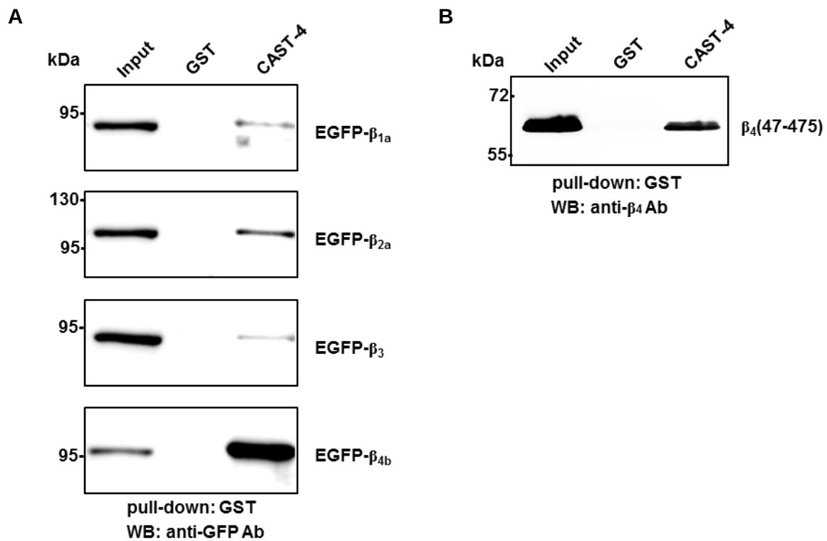
Fig. 2 Direct binding of CAST with VDCC \beta -subunits. (A) GST-pulldown assay of \beta -subunits ( \beta_{1a} , \beta_{2a} , \beta_3 , and \beta_{4b} ) with GST-CAST-4. GST-CAST-4 bound glutathione-Sepharose beads were incubated with cell lysates obtained from EGFP- \beta -transfected HEK293 cells. Bound proteins were analyzed by western blotting using anti-GFP antibody. Ab, antibody; WB, western blotting. (B) In vitro association between the purified GST-CAST-4 and recombinant \beta_4 -subunit ( \beta_4(47-475) ). GST-CAST-4 incubated with \beta_4 -subunit was captured by glutathione-Sepharose beads. Captured \beta_4 -proteins were examined by western blotting.
