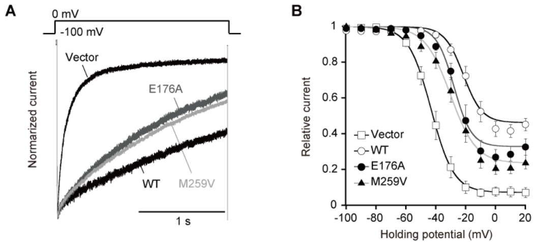
Fig. 3 Autism mutations affect RIM3 regulation of inactivation properties of \text{Ca}_v2.1 VDCCs. (A)
