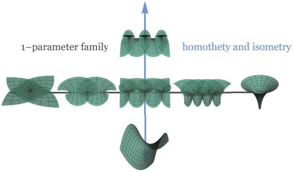
Figure 3: Continuous deformations of ZMC surfaces with planar curvature lines in \mathbb{I}^3 .
