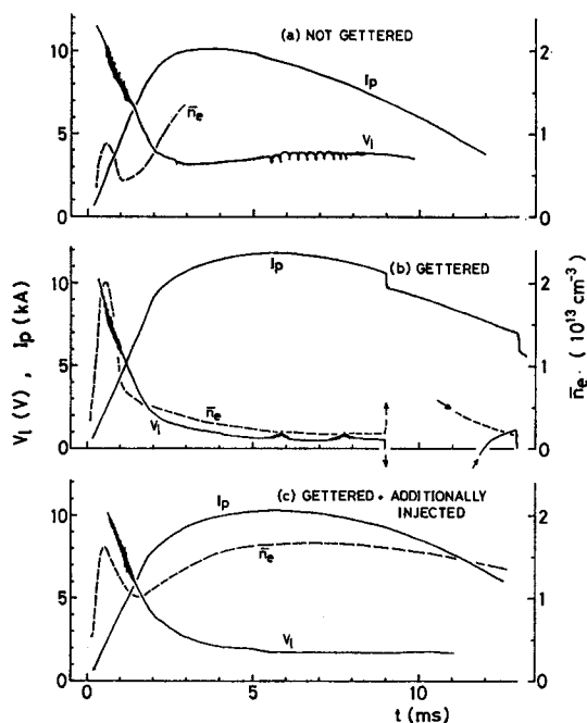
Fig. 2. Typical time dependence of the loop voltage V_l , the plasma current I_p , and the line-averaged electron density \bar{n}_e , in (a) a non-gettered discharge, (b) a gettered discharge with a fast pre-ignition gas puffing, and (c) a gettered discharge with pre-ignition and additional gas puffing.
