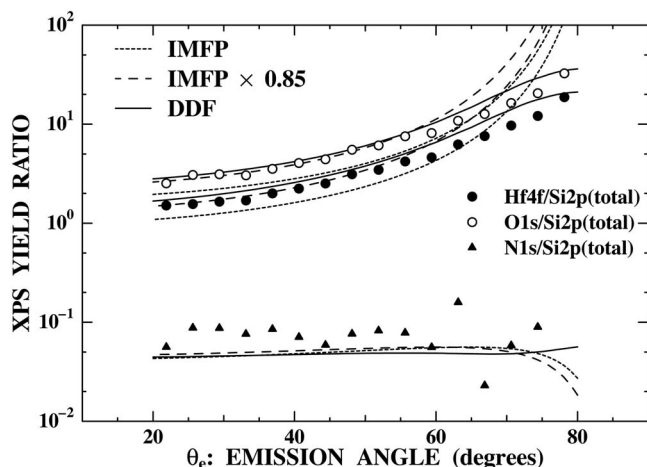
FIG. 2. Comparison between experimental (symbols) and calculated (lines) emission-angle dependences of XPS yields. The yield ratios (\text{Hf } 4f)/(\text{Si } 2p) , (\text{O } 1s)/(\text{Si } 2p) , and (\text{N } 1s)/(\text{Si } 2p) are shown. Calculated results with IMFP (dotted lines), modified IMFP (dashed lines) and DDF (solid lines), are shown.
