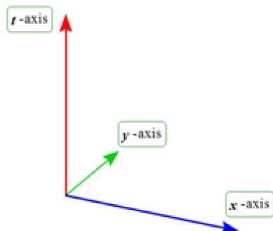
Figure 5. x -axis, y -axis and t -axis
