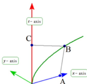
Figure 7. Graph of t = f(x) = \sqrt{x} and points A, B, C (3-dimensional view)
