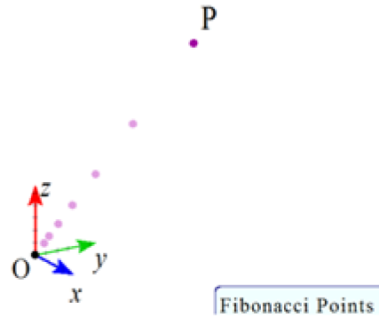
Figure 3. Points P_n
