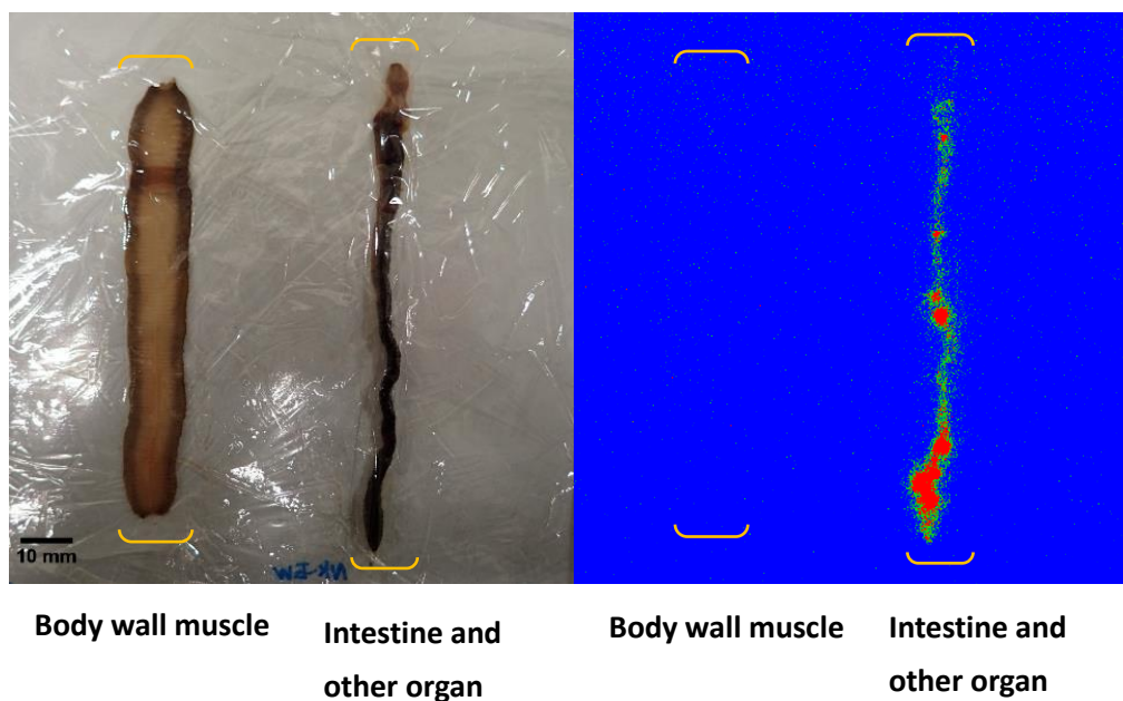
Fig. 4-2 Autoradiographs (right) and photographs (left) of a dissected earthworm. The earthworm was dissected into two parts, body wall muscle and intestine with other organs.
