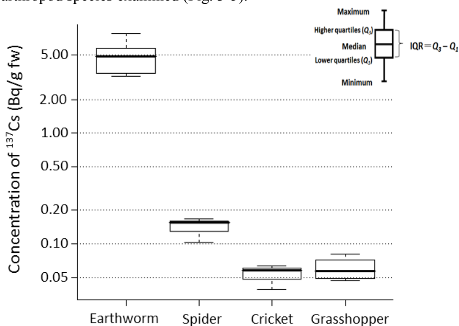
Fig. 3-5 Comparison of radioceium concentration in different feeding habits in 2014.
