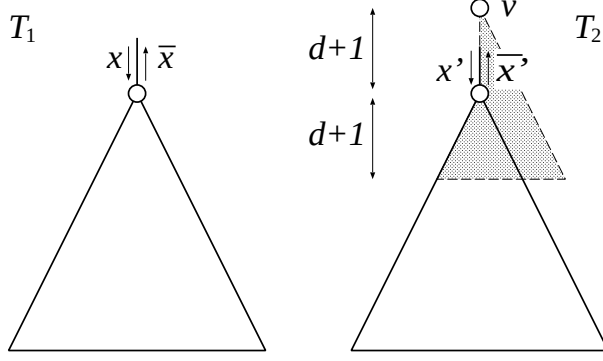
Figure 14: Explanation of Lemma 7. \overline{y'} should be located in the gray region.
