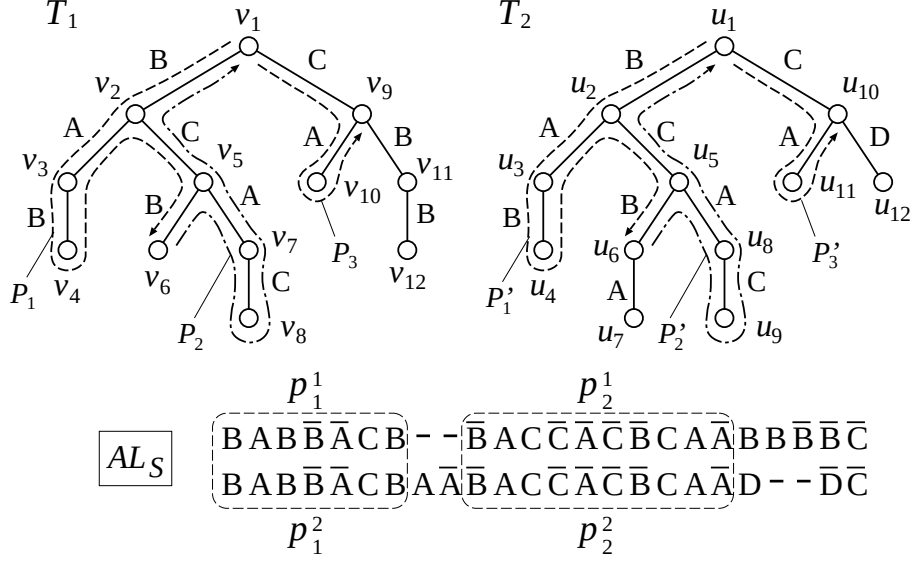
Figure 5: Construction of M_1 from AL_S . Regions surrounded by dashed lines in AL_S correspond to maximal substring pairs. The path corresponding to p_2^1 (resp. p_2^2 ) is divided into P_2 and P_3 (resp. P_2' and P_3' ), where P_2 and P_2' , and P_3 and P_3' are twins respectively. The path corresponding to p_1^1 (resp. p_1^2 ) is divided into P_1 (resp. P_1' ) and an empty path. P_1 , P_1' , P_3 and P_3' are downward paths, whereas P_2 and P_2' are upward paths. P_1 contains central edges of (v_1, v_2), (v_2, v_5), (v_5, v_6) , and P_2 contains central edges of (v_6, v_5), (v_5, v_2), (v_2, v_1) . M_1 = \{(v_2, u_2), (v_3, u_3), (v_4, u_4), (v_5, u_5), (v_6, u_6), (v_9, u_{10}), (v_{10}, u_{11})\} .
