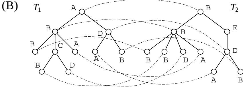
Figure 1: (A) Insertion and deletion operations. (B) T_2 is obtained by deletion of a node with label ‘C’, insertion of a node with label ‘E’ and substitution for the root node. A mapping corresponding to this edit sequence is also shown by dashed curves.
