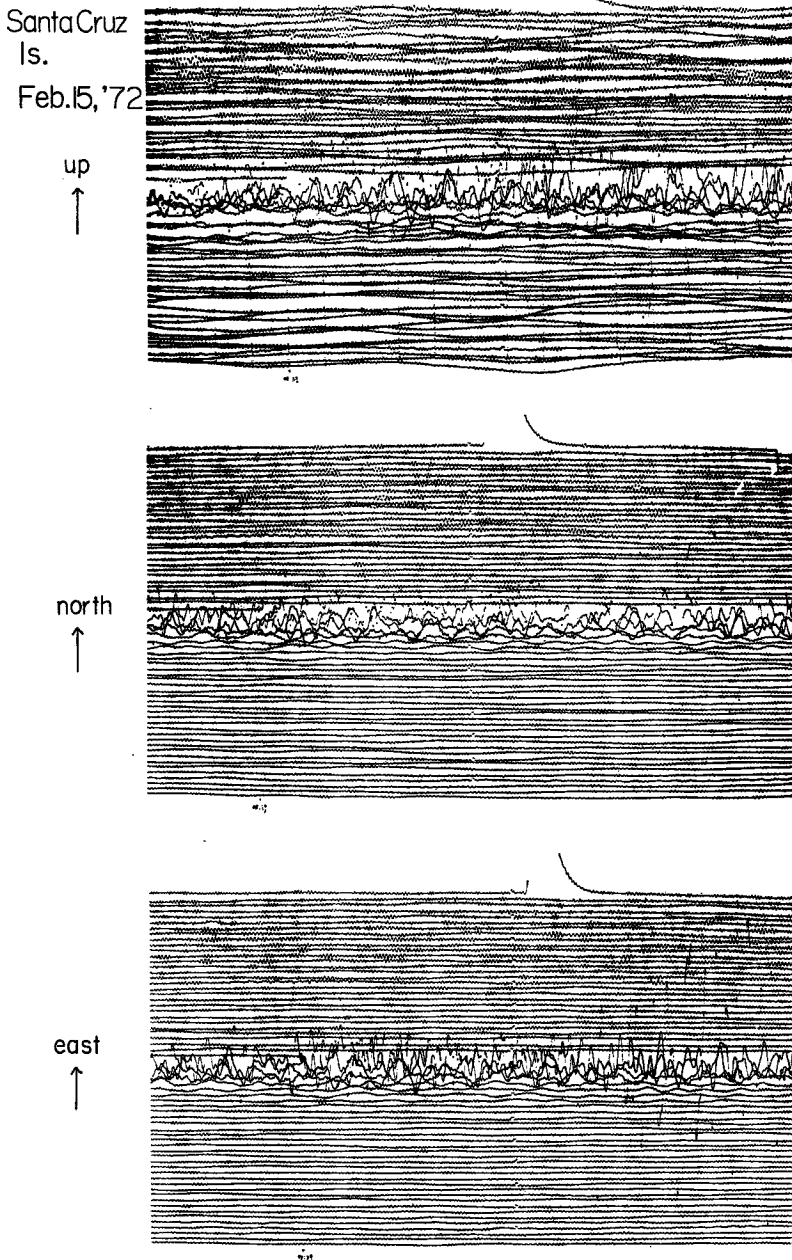
Fig. 5 The same seismogram as Fig. 4 by conventional Press-Ewing seismograph system.
