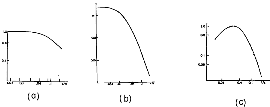
Fig. 2 Amplitude frequency response curves of OP-amp., filter, and seismograph system.
