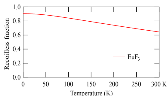
Fig. 1. Calculated Recoilless fraction of Mössbauer effect for ^{151}\text{Eu} nuclear resonance at \text{EuF}_3 .
