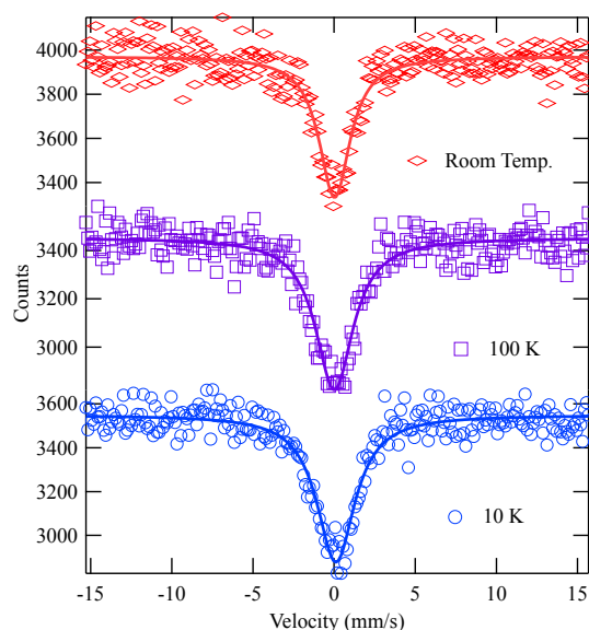
Fig. 2. ^{151}\text{Eu} Mössbauer spectra of \text{EuF}_3 at some temperatures.
