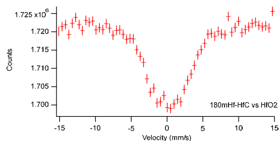
Fig. 2. ^{180}\text{Hf} -Mössbauer spectrum of \text{HfO}_2 using ^{180\text{m}}\text{Hf} source in HfC at 22K.
