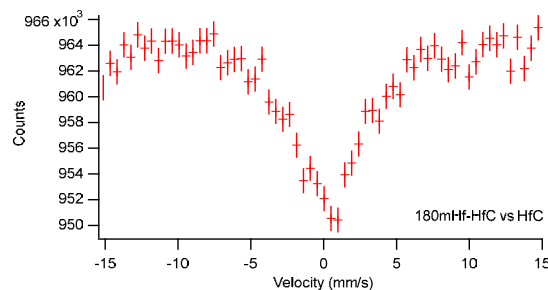
Fig. 1. ^{180}\text{Hf} -Mössbauer spectrum of HfC using ^{180\text{m}}\text{Hf} source in HfC at 22K.
