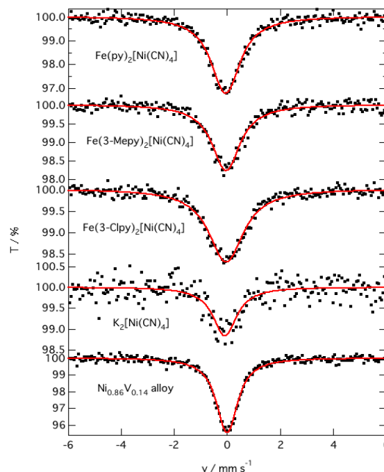
Fig.1 61 Ni Mössbauer Spectroscopy for Supramolecular Bridging Cyanide Complexes.
