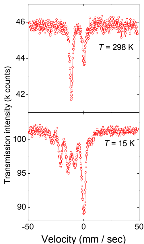
Fig. 1. ^{151}\text{Eu} Mössbauer spectra for \text{EuSn}_2\text{P}_2 at temperatures ( T ) = 15 K and 298 K.
