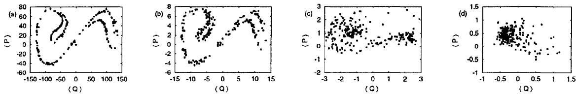
Figure 1: These are the stroboscopic maps for (\langle\hat{Q}\rangle, \langle\hat{P}\rangle) . The each point in these figures represents the data at every 2\pi/\Omega for a single realization of complex Wiener process. Figures (a), (b), (c) and (d) are for \beta = 0.01, 0.10, 0.40 and 1.00 , respectively.
