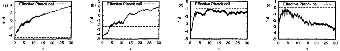
Figure 2: These figures are the time evolution of \Delta(\tau) with \epsilon fixed as 0.01. The complex Wiener process is used in QSD. Figures (a) and (b) are obtained with single realization of complex Wiener process for each initial condition (20 samples). Figures (c)–(d) are obtained with averaging over 100 realizations of complex Wiener process for each initial condition (10 samples). Figures (a), (b), (c) and (d) are for \beta = 0.01, 0.10, 0.40 and 1.00 , respectively.
