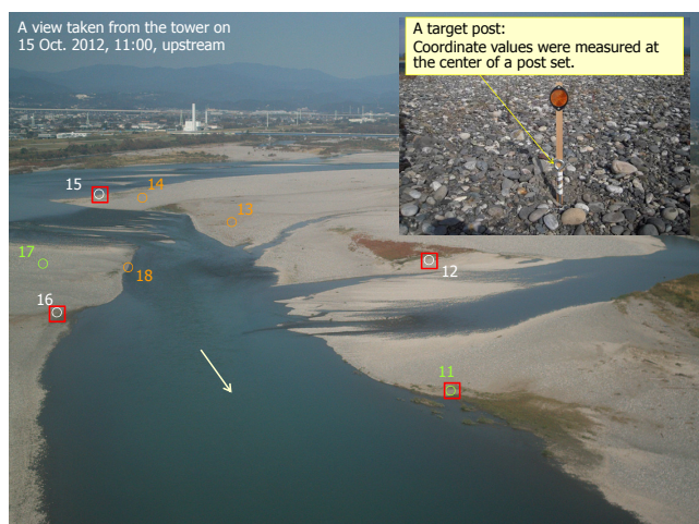
Fig. 14 Data transformed into the ortho data through the photogrammetric method. “○” in the fig. refers to a location where target posts having coordinate values have been set. 2D ortho data were developed based on No. 11, 12, 15, and 16, referred to as “□” in the fig., using a photogrammetric method.
