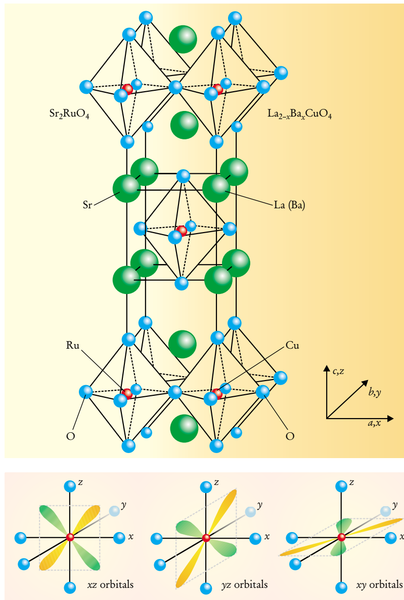
FIGURE 1. STRONTIUM RUTHENATE ( \text{Sr}_2\text{RuO}_4 ) forms a layered perovskite structure. As shown in the upper panel, the crystal's \text{RuO}_6 layers are separated by \text{Sr} layers, and each \text{Ru} ion is enclosed in an octahedral cage of oxygen ions. The same structure is also found in \text{La}_2\text{CuO}_4 , which is the parent compound of the high- T_c superconductor \text{La}_{2-x}\text{Ba}_x\text{CuO}_4 . Despite their structural similarity, the ruthenate and the cuprate have very different electronic properties: \text{Sr}_2\text{RuO}_4 is strongly metallic and a superconductor at low temperature, whereas \text{La}_2\text{CuO}_4 is an antiferromagnetic insulator. The lower panel shows the configuration of the orbitals responsible for the superconductivity of \text{Sr}_2\text{RuO}_4 , namely, the 4d t_{2g} orbitals.
