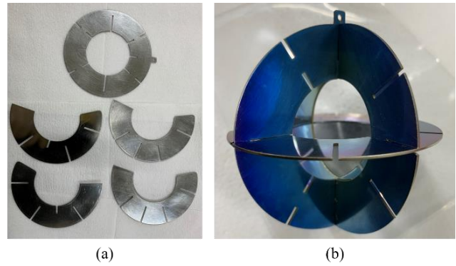
Fig. 1. The SUS304 plates for cathodes (a), and the Ti-coated cathode after assembly (b)
