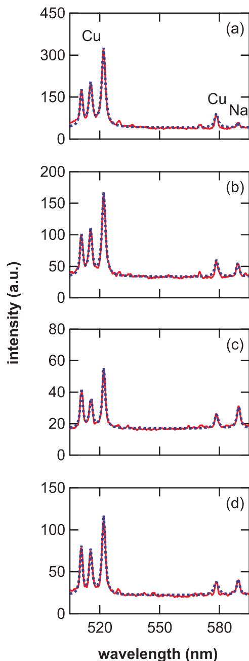
FIG. 5. Emission spectra (solid line) of the laser ablation plasma produced on a Cu plate in 5 mM NaCl aqueous solution and the best-fit theoretical spectra (broken line). The results (a)–(d) show the emission spectra obtained at each position (A)–(D), respectively. The pulse width was 100 ns and the pulse energy was 6 mJ. The emission spectra were measured at the delay time of 1000 ns from the laser irradiation. The gate width of the ICCD was set to 650 ns.
