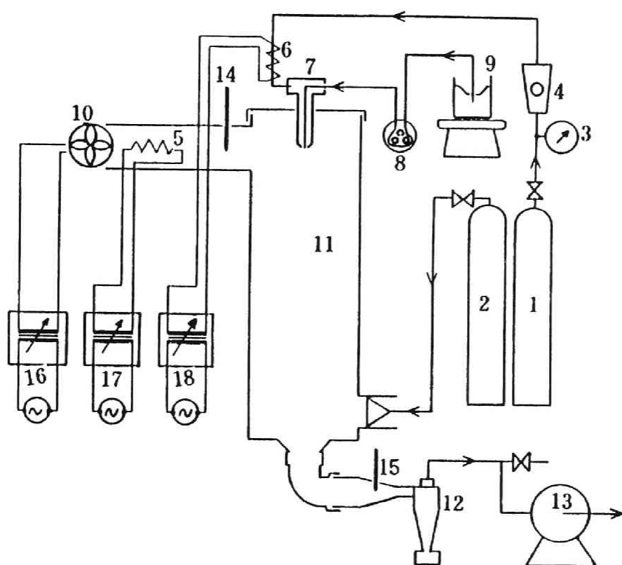
Figure 2-1. Schematic diagram of spray drying tower.
