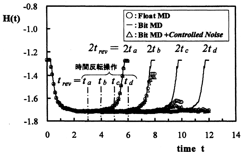
Fig.1 Time evolution of H-function.
