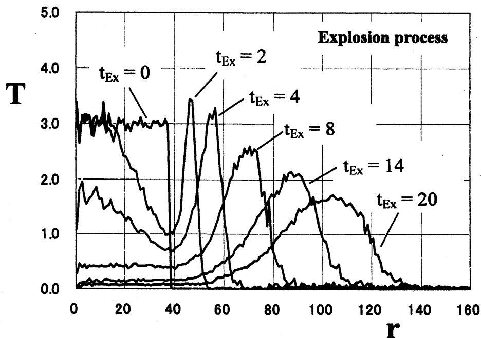
Fig. 2 Radial distributions of thermal temperature (Explosion).
