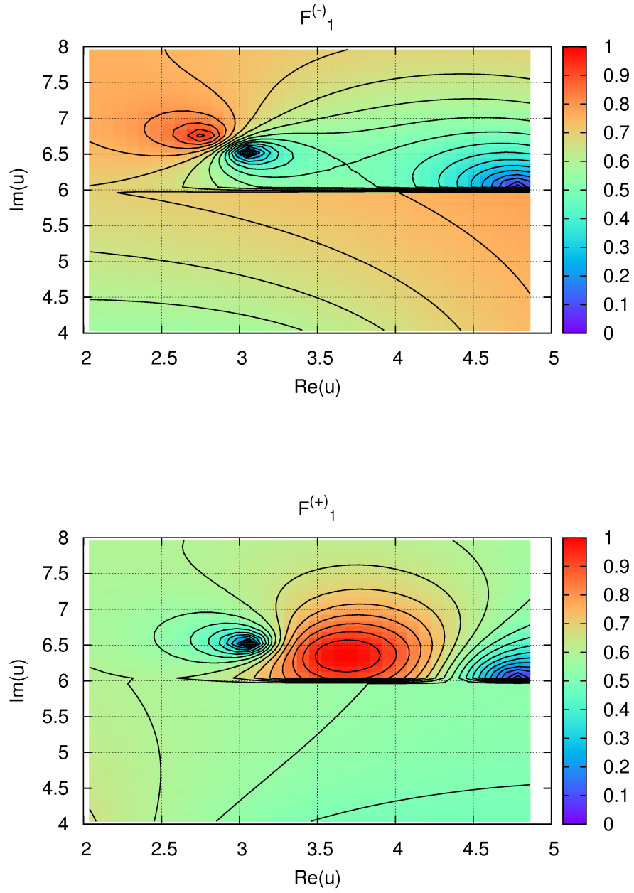
Figure 21. Details of F_1^\pm(u) : L = 4 , g = 0.5 , \mu_y = 0 .
