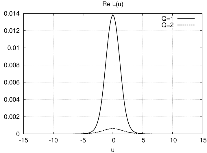
Figure 7. Solutions \text{Re}(L_Q) : L = 4 , g = 0.5 , \mu_y = 0 .
