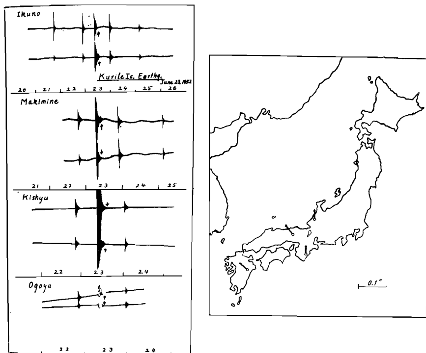
Fig. 6 Tiltgrams disturbed by Kurile Islands Earthquake on June 23, 1952.
