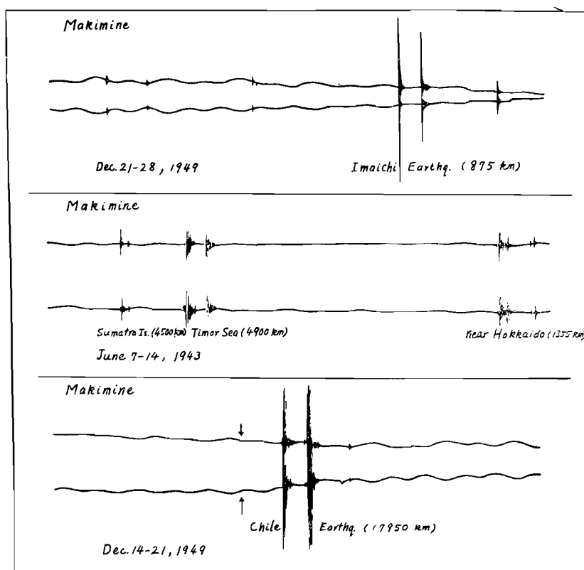
Fig. 2 Examples of tiltgrams disturbed by the far distant earthquakes at Makimine Station.
