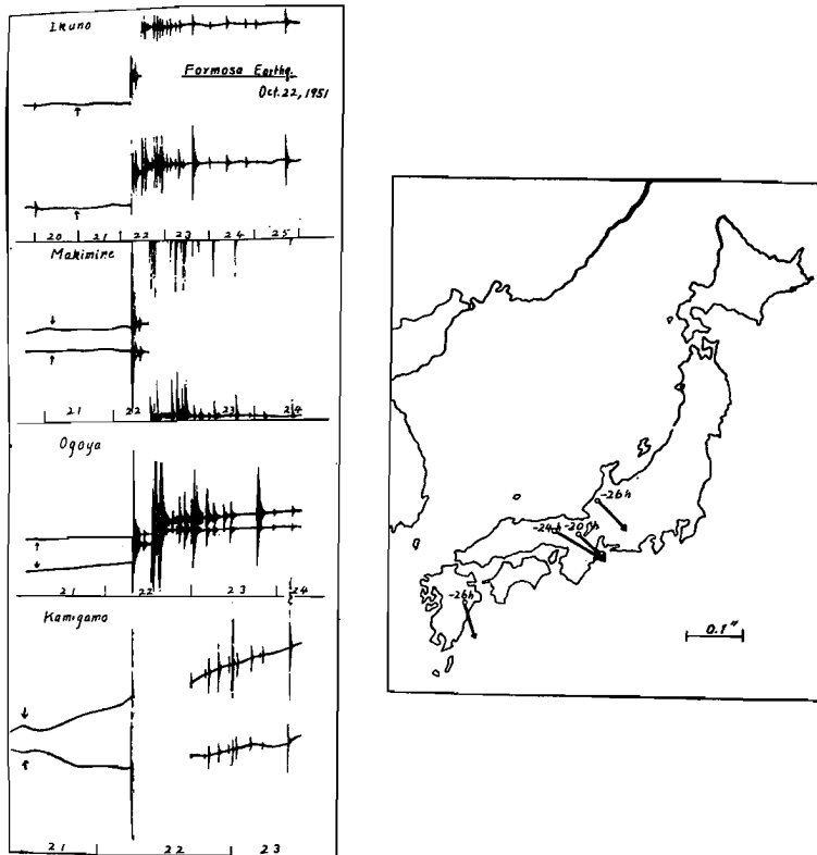
Fig. 5 Tiltgrams disturbed by Formosa Earthquake on October 22, 1951.
