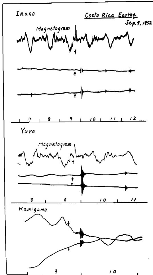
Fig. 7 Tiltgrams and magnetogram disturbed by Costa Rica Earthquake on September 9, 1952.
