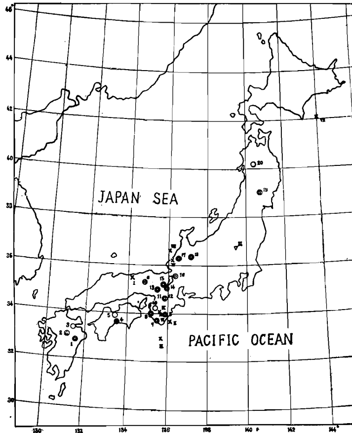
Fig. 1 Observation Stations.
