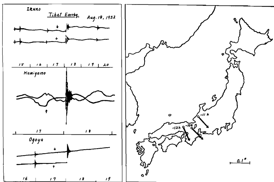
Fig. 3 Tiltgrams disturbed by Tibet Earthquake on August 18, 1952.
