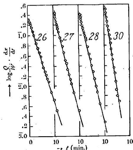
Fig. 10. Influence of hydrogen gas on the nitrogen sol. (a).
