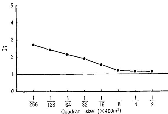
Fig. 4. I_s -Quadrat size relation for distribution of total germinant Hinoki seedlings in 1974.
