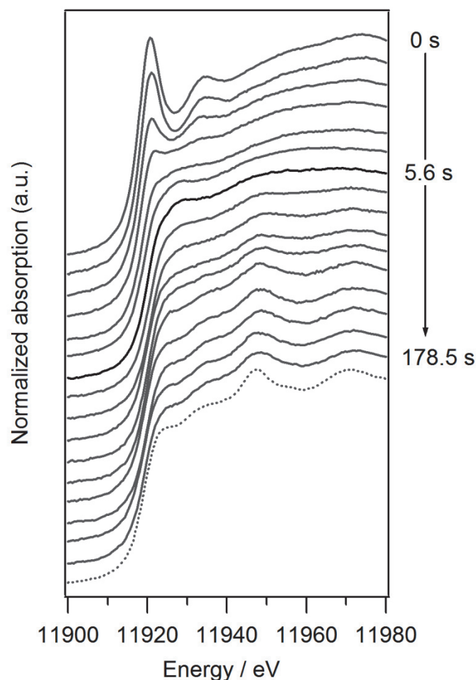
Figure 6. Series of XANES spectra during \text{H[AuCl}_4\text{]} reduction in the presence of 1 (solid line), together with the spectrum of Au foil (dotted line). The black solid line represents Au nuclei at 5.6 s.
