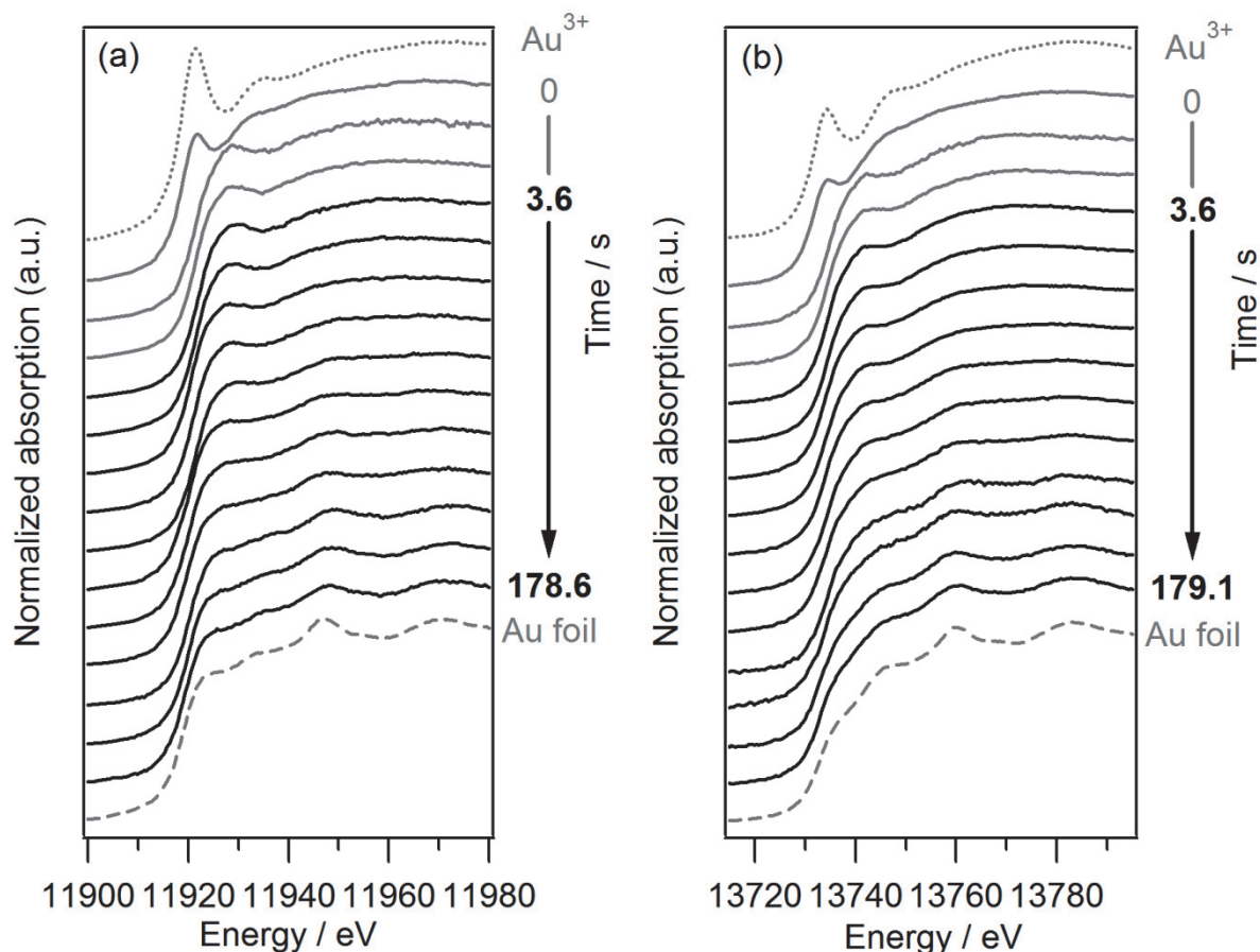
Figure 1. The series of XANES spectra at (a) Au L_3 and (b) L_2 edge during particle formation (solid lines), together with those of HAuCl_4 in DMF ( Au^{3+} solution) (dotted line) and Au foil (dashed line). The series of spectra during particle formation and that of Au^{3+} solution were shifted vertically for clarity.
