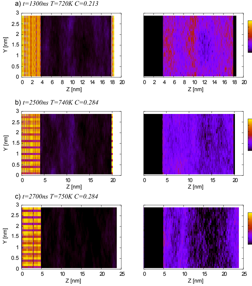
Fig. 9 Number density maps at 450bar. Left and right figures show the number densities of ions and water, respectively.
