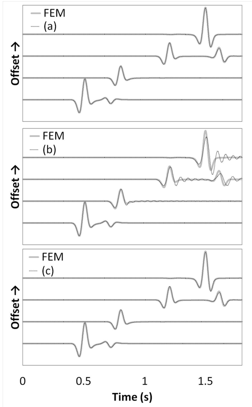
Figure 15. Waveforms obtained by different arrangement of calculation points compared with FEM. Upper, middle and lower figures show the comparison between the fine, coarse, partially fine arrangements and FEM, respectively.
