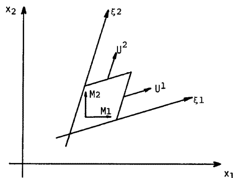
Fig. 2. Cartesian coordinate system and generalized curvilinear coordinate system.
