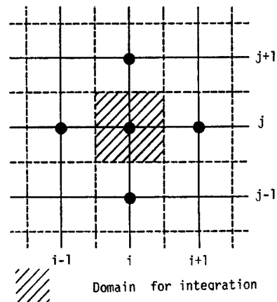
Fig. 4. Definition of locations of variables and finite difference grids in generalized curvilinear coordinate system.
