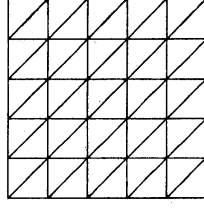
Figure 1: Triangular meshes of Friedrichs-Keller type for a square domain
