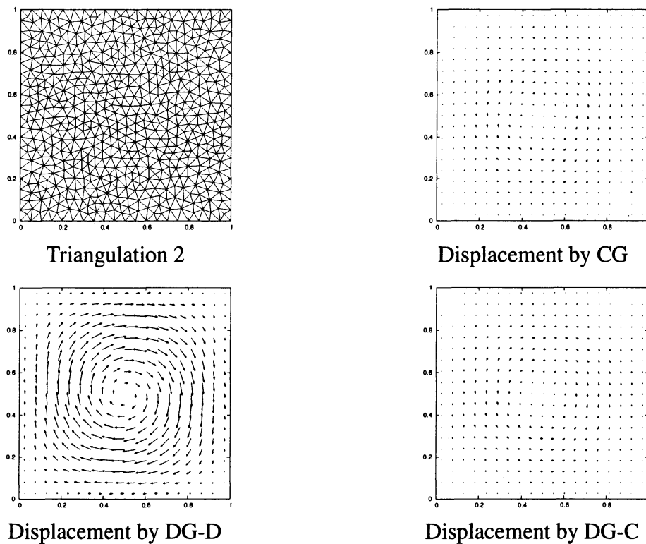
Figure 6: Triangulation 2 and computed displacements
