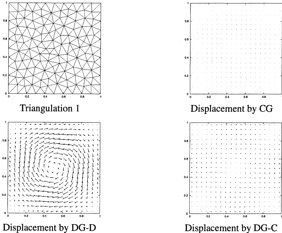
Figure 5: Triangulation 1 and computed displacements
