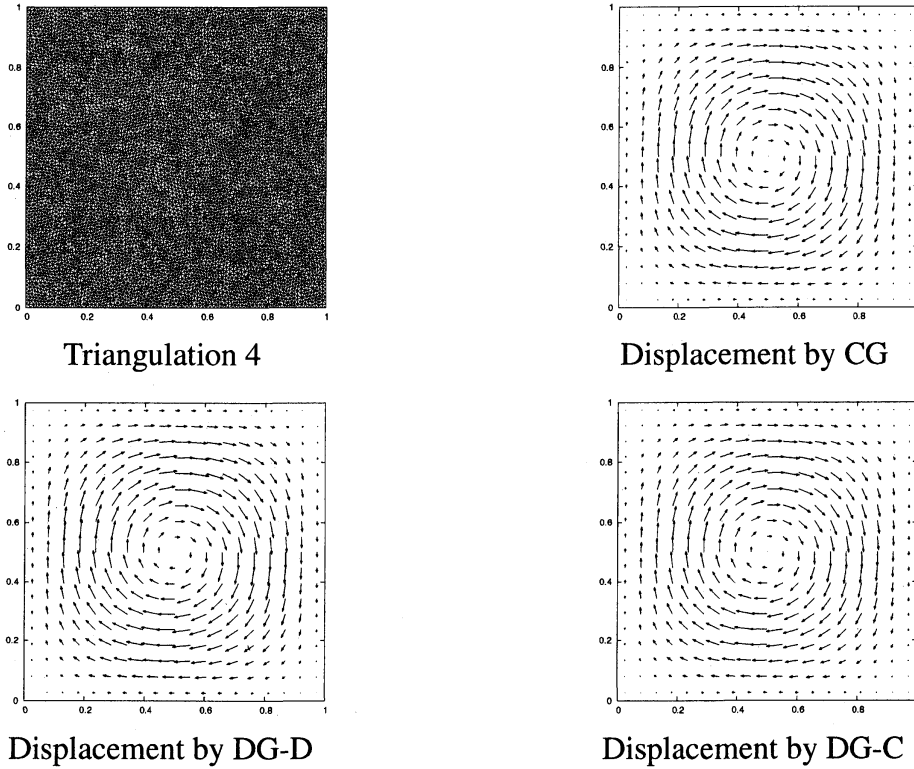
Figure 8: Triangulation 4 and computed displacements
