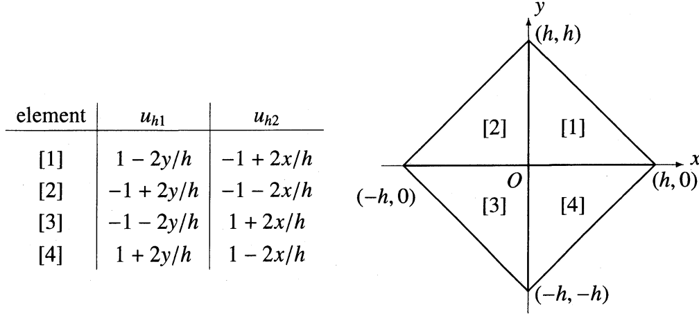
Figure 4: Example of patch of triangular elements
