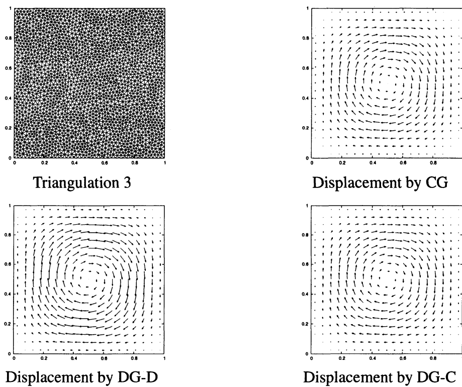
Figure 7: Triangulation 3 and computed displacements
