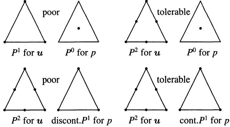
Figure 2: Some combinations of u and p for triangles
