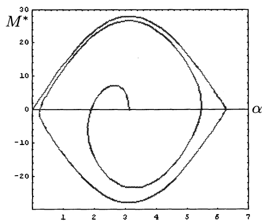
Fig 8: Torque curve for K = 14
