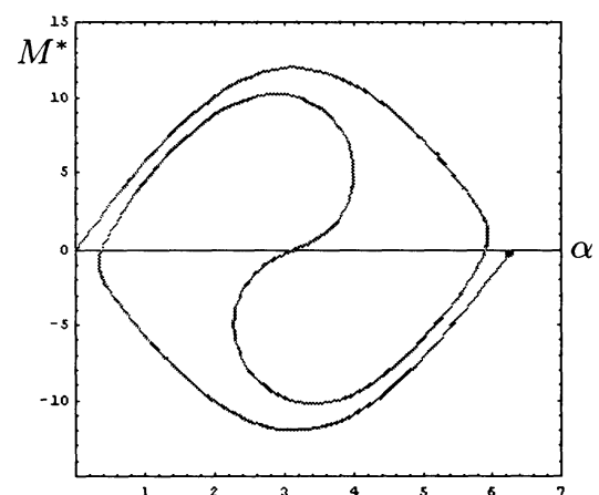
Fig 5: Torque curve for K = 6
