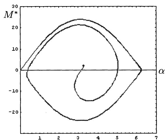
Fig 7: Torque curve for K = 12
