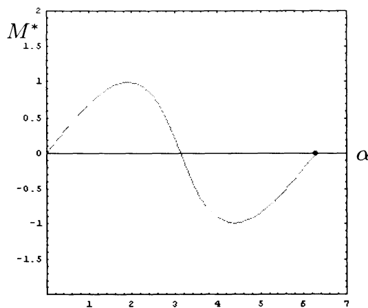
Fig 2: Torque curve for K = 1
