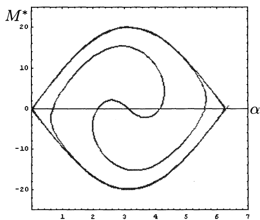
Fig 6: Torque curve for K = 10
