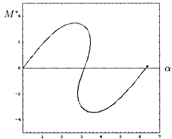
Fig 3: Torque curve for K = 2
