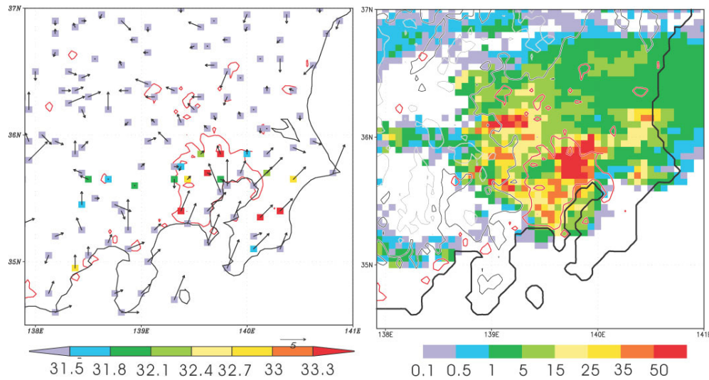
Fig.1 (a) Averaged surface temperature for 12-14 JST with the AMeDAS, and (b) accumulated rainfall for 15-18 JST with the Rader-AMeDAS on 21 July 1999. TMA is surrounded by the red line.
