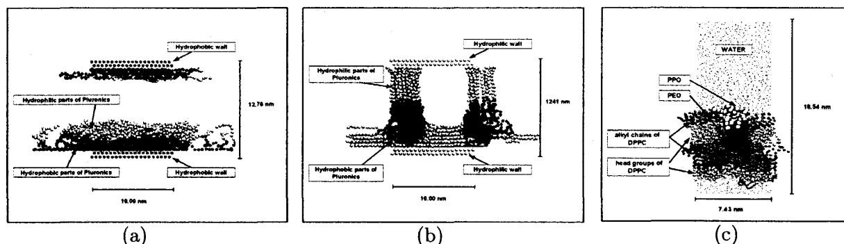
Figure 1: Snapshots of Pluronics. PPO monomers are shown in black and PEO in white, water is not shown for clarity at (a) and (b). Periodic boundary condition is applied. (a): Pluronics and hydrophobic walls, (b): Pluronics and hydrophilic walls, (c): Pluronics and DPPC bilayer.
