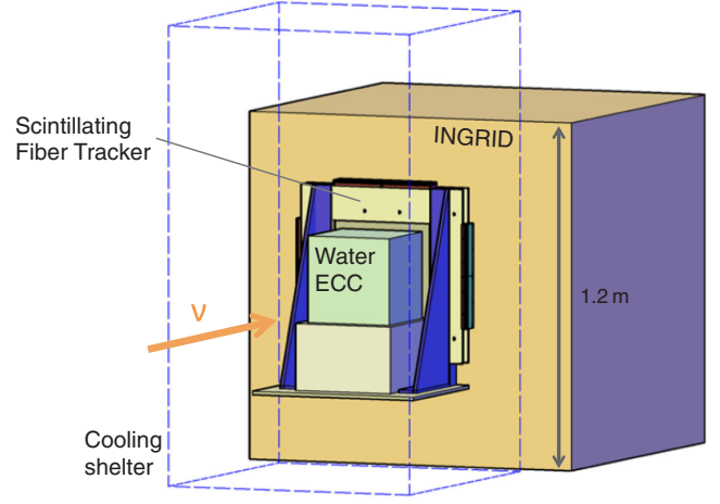
FIG. 1. Schematic view of the detectors. The ECC and SFT are installed in a cooling shelter, which is placed in front of an INGRID module.
