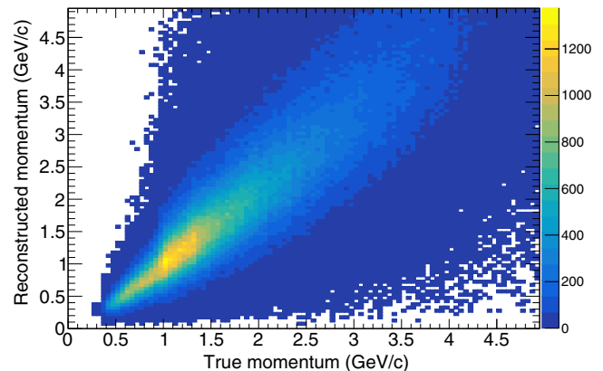
FIG. 7. Relation between the true and reconstructed momenta of muons from neutrino interactions in the MC simulation.
