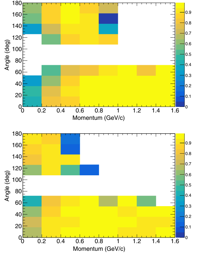
FIG. 10. Proton (top) and pion (bottom) detection efficiencies estimated by the MC simulation.
