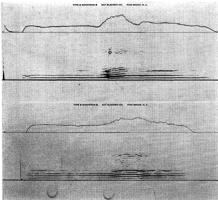
Fig. 7 Sonagrams illustrating the effects of increased exhalation on the pitch. upper : amplitude of voice, lower : frequency spectrum analysed by narrow band pass filter
