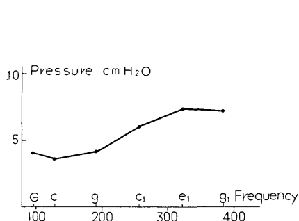
Fig. 4 Minimal subglottic pressure required for phonation at given pitch. Vowel "ah" is sung, the subject male.
