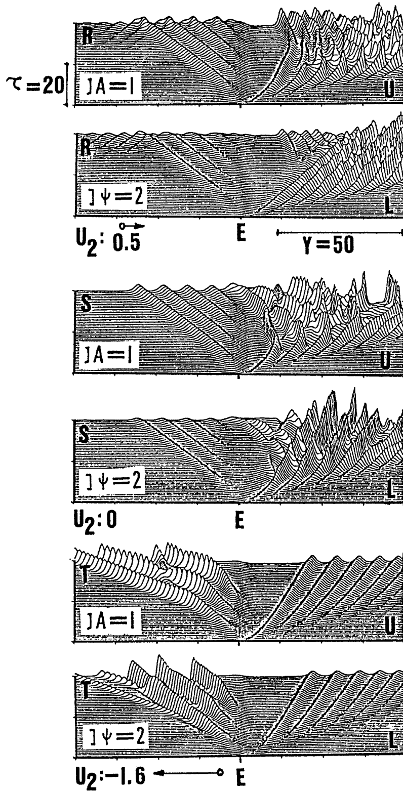
Fig. 2. Time evolution of variations of the upper and lower layers (U and L) around a cape. 1) R (top) for a positive flow in the lower layer, 2) S (middle) for no flow in the lower layer, 3) T (bottom) for negative flow in the lower layer.
