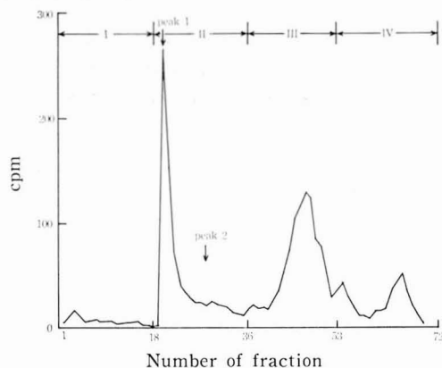
Fig. 3. Ion-exchange chromatogram of the aqueous metabolites on Dowex 1-X8. The sample is the metabolites in S strain 4 hr after topical application of malathion ( 1.0 \mu\text{g} per female). A series of gradient elution is as following as described by Krueger and O'Brien 26 ). Three hundred ml of each gradient eluant was used. Gradient I: HCl pH 1.5/HCl pH 1, Gradient II: HCl pH 2 + methanol (1+4)/HCl pH 1 + methanol (1+4), Gradient III: HCl pH 1 + methanol (1+3)/HCl 1 N + methanol (1+3), Gradient IV: HCl 1 N + acetone (1+3)/HCl conc. + \text{H}_2\text{O} + acetone (1+1+6).
