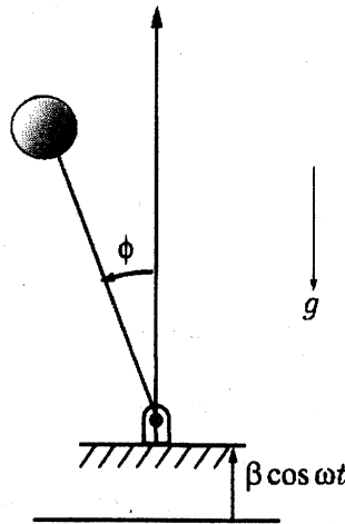
Figure 1: Vertically excited pendulum
