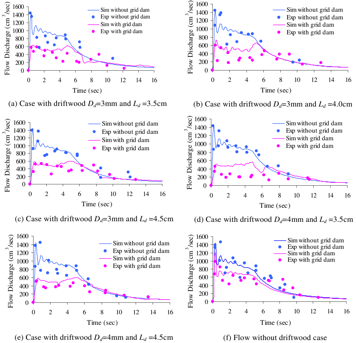
Fig. 23 Flow discharge at downstream end of flume and discharge reduction by grid dam due to driftwood jamming
