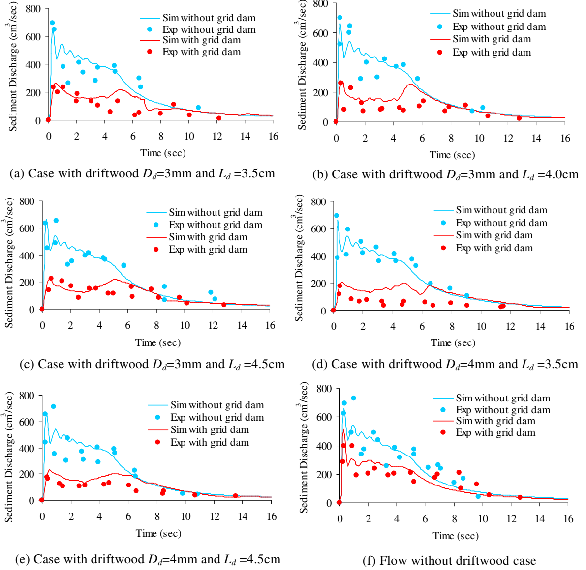
Fig. 24 Sediment discharge at downstream end and discharge reduction by grid dam due to driftwood jamming
