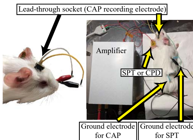
Fig. 3. The setting of compound action potential (CAP) measurement. SPT: a skin-mediated piezoelectric transducer. CPD: a conventional piezoelectric diaphragm
