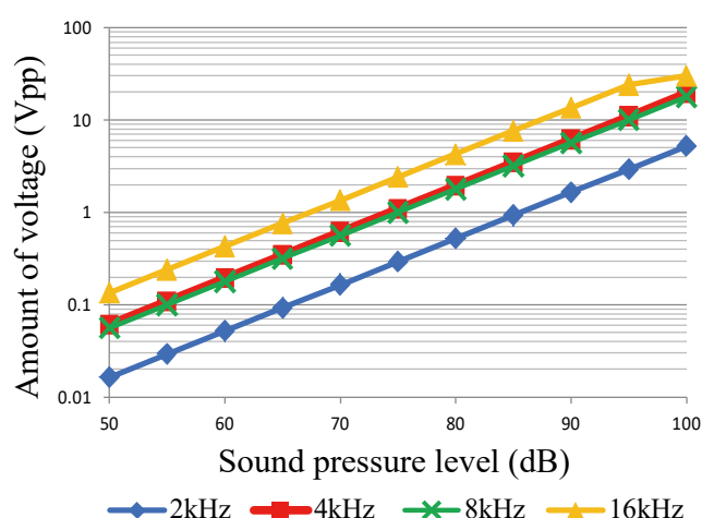
Fig. 4. The relationship between the amounts of voltage applied to the SPT or CPD and the sound pressure level
