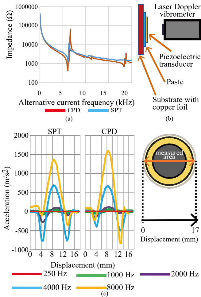
Fig. 5. The comparison of material characteristics between conventional and novel piezoelectric transducers. The electrical (a) and vibratory (b and c) characteristics of both transducers were evaluated. The electrical and vibration behaviors of both the skin-mediated piezoelectric transducer (SPT) and conventional piezoelectric diaphragm (CPD) were similar for each frequency.
