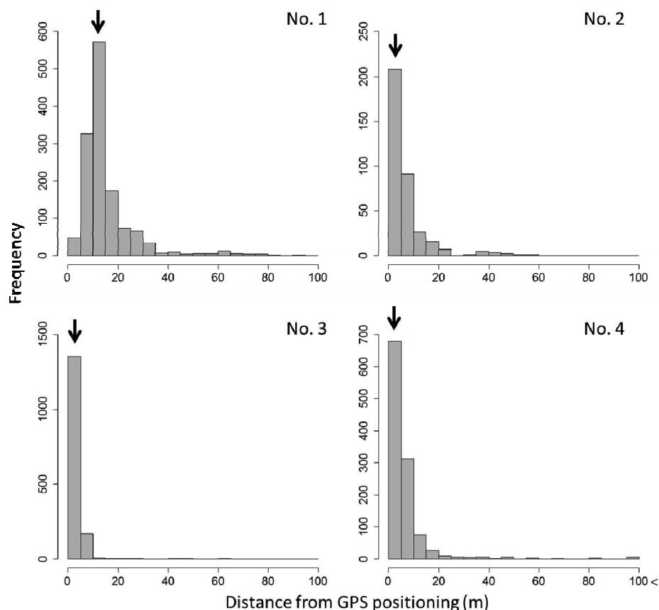
Fig. 6. Distance between VPS results of fixed transmitters and GPS positioning. Arrows indicate the highest number of localizations.
