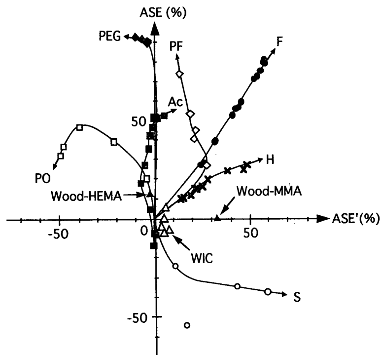
Fig. 2. Relationships between the ASE and ASE' values for nine kinds of chemical treatments of hinoki wood.
