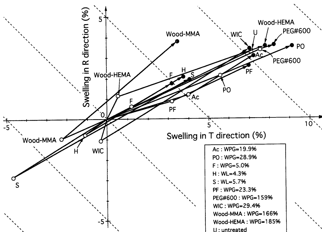
Fig. 1. Relationships between swelling coefficients in R and T directions.
