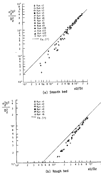
Fig. 7 (a), (b) Relation between \sigma_z^2 and x .
