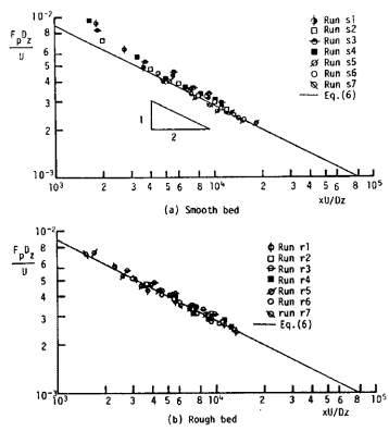
Fig. 19 (a), (b) Relation between F_p and x .
