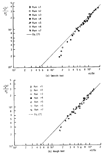
Fig. 20 (a), (b) Relation between \sigma_z^2 and x .
