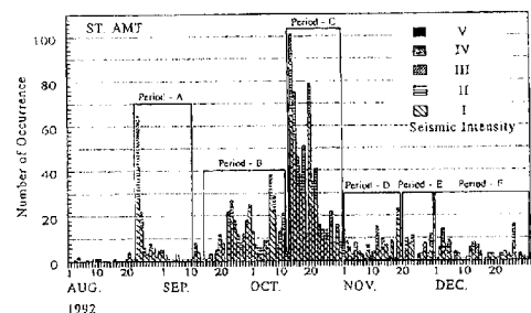
Fig.7 Daily frequency distribution of felt earthquakes at the station AMT from August to December in 1992. Periods A-F correspond to epicenter maps (b)-(g) in Fig.8.
