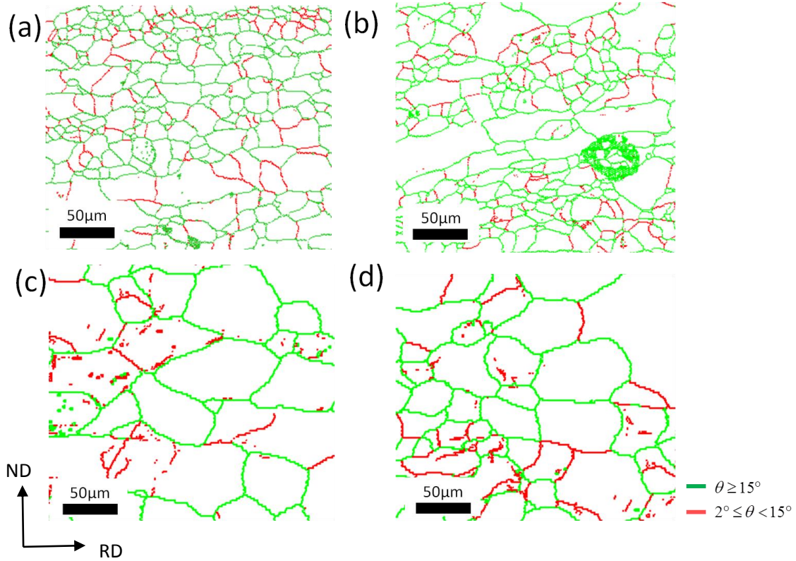
Figure 2.2 EBSD grain boundary maps of (a) 90% cold rolled + 650°C annealed + air-cooled ( d=13.6\mu\text{m} ), (b) 90% cold rolled + 650°C annealed + water-cooled ( d=15.2\mu\text{m} ), (c) 50% cold rolled + 800°C annealed + air-cooled ( d=41.8\mu\text{m} ) and (d) 50% cold rolled + 800°C annealed + water-cooled ( d=45.1\mu\text{m} ) specimens.
