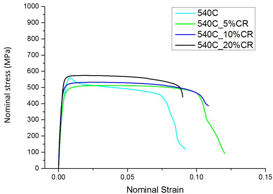
Figure 3.19 Stress-strain curves of the specimen with d=0.8 \mu\text{m} , after post-annealing cold rolling by different reductions.
