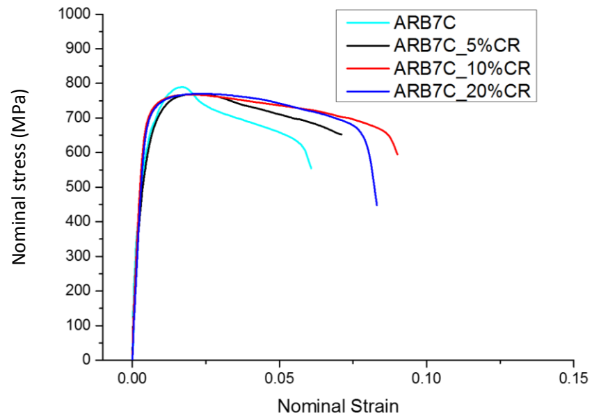
Figure 3.16 Stress-strain curves of the as-ARB processed specimen and ARB processed and cold-rolled specimen.
