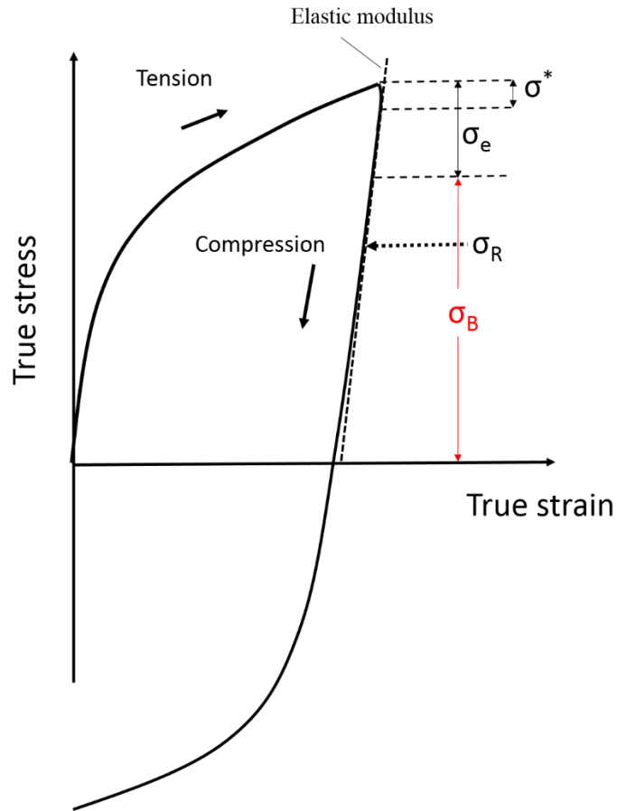
Figure 4.7 Illustration showing the measurement way of the back stress ( \sigma_{Back} ) from the tension-compression test.
