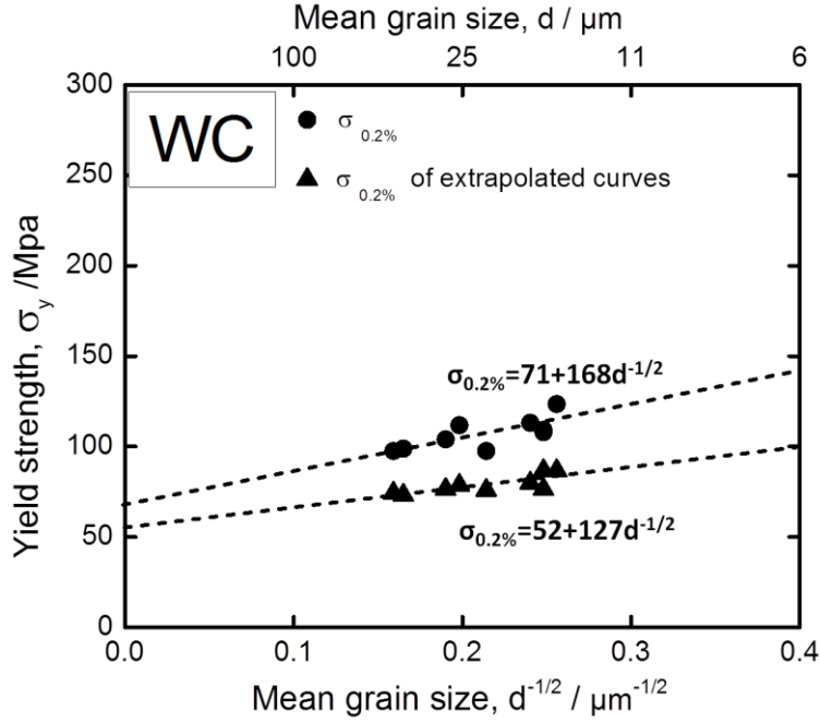
Figure 2.15 The \sigma_{0.2\%} measured from the stress-strain curves of the WC specimens are plotted against d^{-1/2} . The Hall-Petch relationship is also given.
