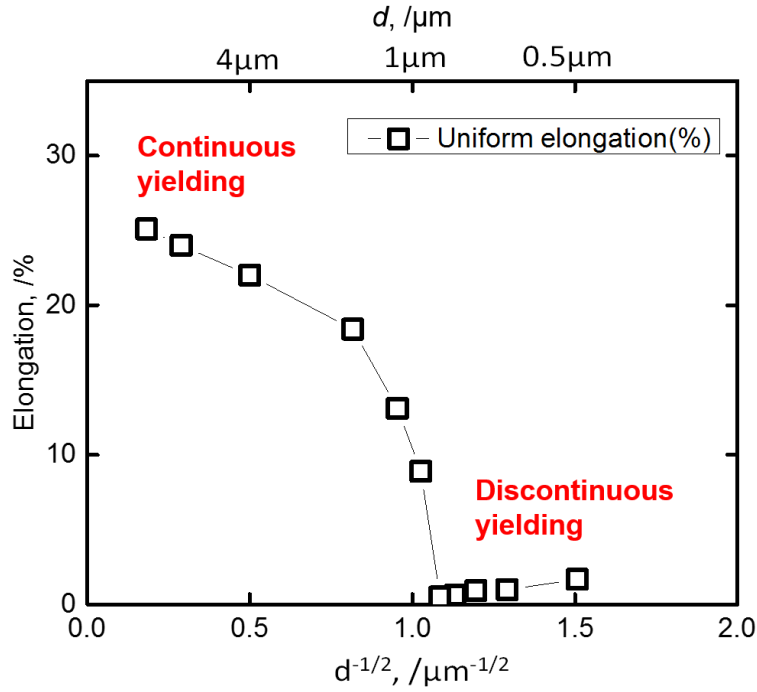
Figure 3.5 Uniform elongation of the IF steel specimens plotted as a function of inverse square root of the mean grain size. A dramatic drop in the uniform elongation occurs in the range 0.45 \mu\text{m} < d < 0.9 \mu\text{m} .
