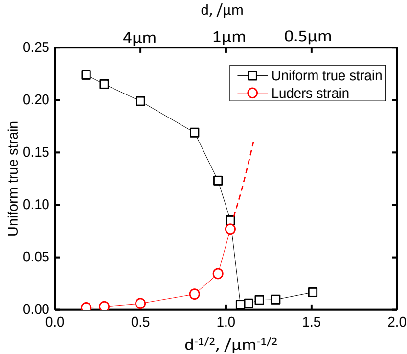
Figure 3.12 True strain corresponding to the uniform elongation and the maximum local strain obtained from the DIC analysis at 2% plastic tensile strain of the specimens having different grain sizes are plotted against d^{-1/2} . The dramatic increasing of the local strain in the fine grain size range can be seen.
