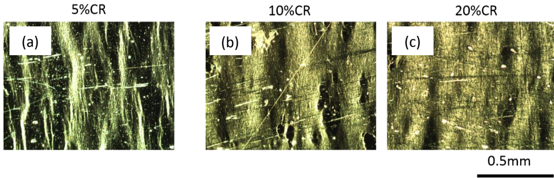
Figure 3.15 Optical micrographs showing the surface morphologies of the ARB+540°C annealed specimen with d=0.8 \mu\text{m} after post-annealing cold rolling by (a) 5%, (b) 10% and (c) 20%..
