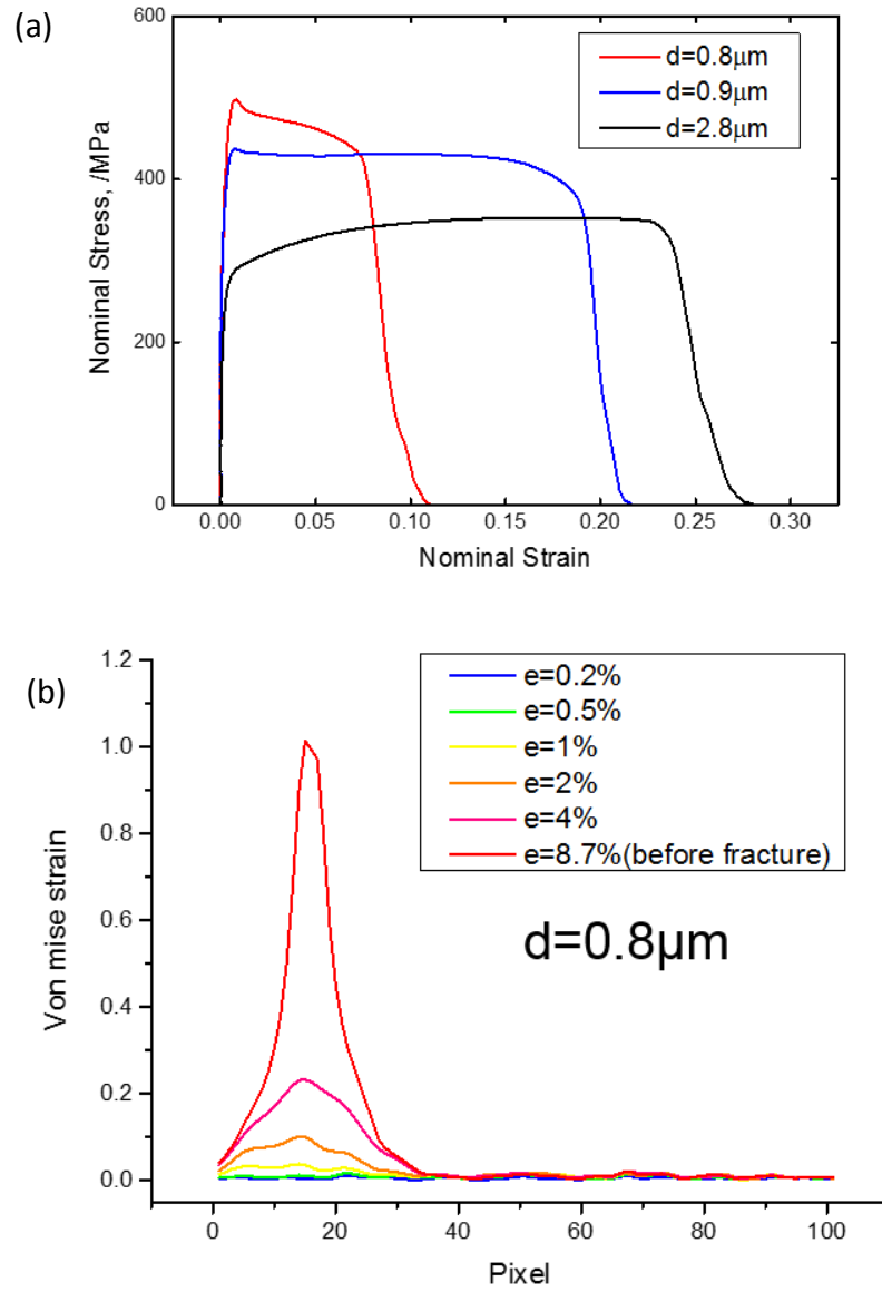
Figure 3.10 (a) Representative stress-strain curves of the specimens having different mean grain sizes. (b~d) The strain distribution plots during tensile test of the specimens having (b) d=0.8\mu\text{m} (c) d=0.9\mu\text{m} and (d) d=0.8\mu\text{m} .
