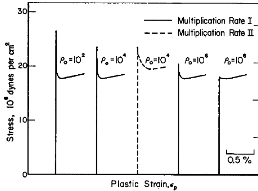
Figure 1.4 Calculated stress-strain curves by Hahn's model showing the influence of the initial dislocation density on the yield drop in a low carbon steel. \rho_0 is the initial dislocation density in an unit of \text{cm}^{-2} [4]. The corresponding initial dislocation density \rho_0 is 10^2\text{cm}^{-2} , 10^4\text{cm}^{-2} , 10^4\text{cm}^{-2} , 10^6\text{cm}^{-2} , 10^8\text{cm}^{-2} from left hand side to right hand side, respectively.
