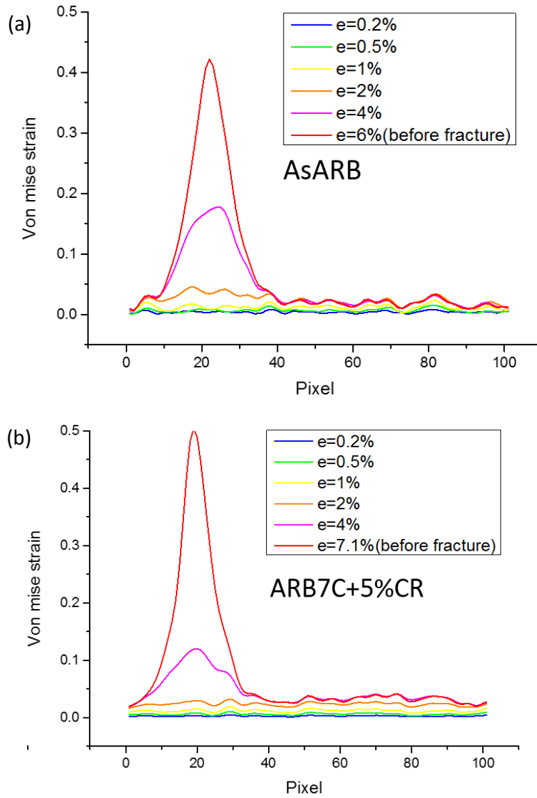
Figure 3.18 Strain distribution maps of the (a) as-ARB specimen and the ARB processed specimen cold-rolled by (b) 5%, (c) 10% and (d) 20%
