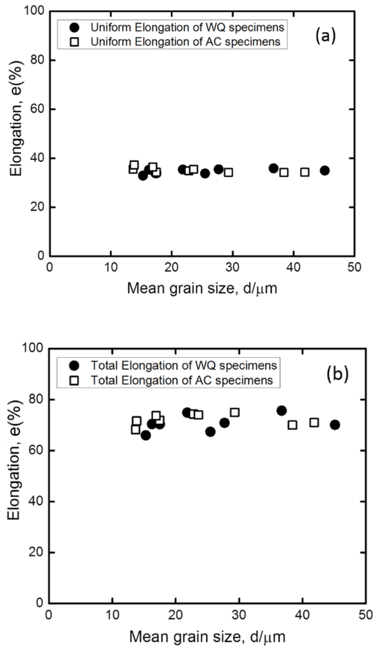
Figure 2.5 Uniform elongation (a) and total elongation (b) as a function of the mean grain size for the water-cooled and air-cooled specimens.
