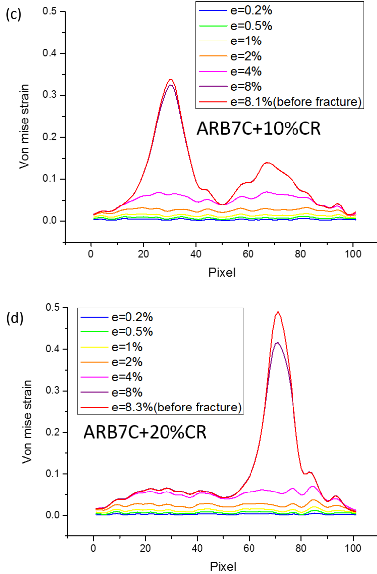
Figure 3.18 (Continued) Strain distribution maps of the (a) as-ARB specimen and the ARB processed specimen cold-rolled by (b) 5%, (c) 10% and (d) 20%
