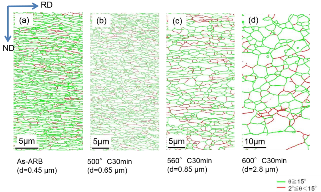
Figure 3.2 EBSD boundary maps of the IF steel specimens ARB processed to an equivalent strain of 4.8 and subsequently annealed at various temperatures for 1.8 ks. (a) As ARB processed. (b) Annealed at 500°C. (c) Annealed at 560°C. (d) Annealed at 600°C.
