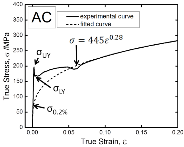
Figure 2.12 The extrapolation process on an AC specimen is shown. Dashed line represents the extrapolated stress-strain curve according to Hollomon's formula, from which the \sigma_{0.2\%} can be determined.
