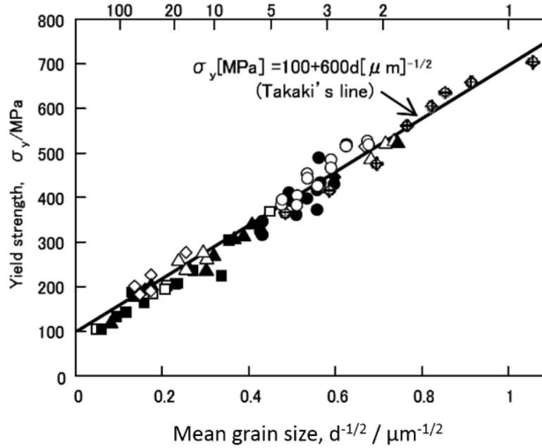
Figure 2.11 The Hall-Petch relationship for several low carbon steels [5].
