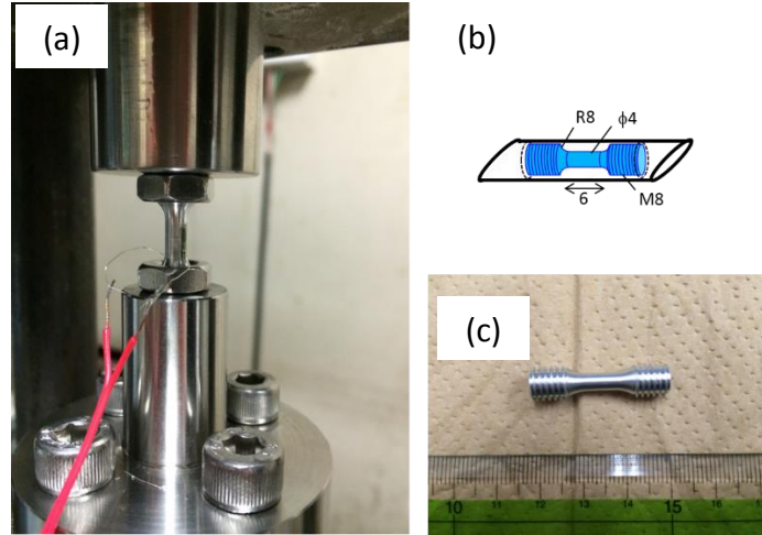
Figure 4.6 Photographs and illustration showing (a) the setting of the Bauschinger test specimen (b) the dimension of the specimen, and (c) the specimen.
