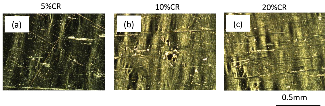
Figure 3.14 Optical micrographs showing the surface morphologies of the as-ARB specimen after cold rolling by (a) 5%, (b) 10% and (c) 20%.
