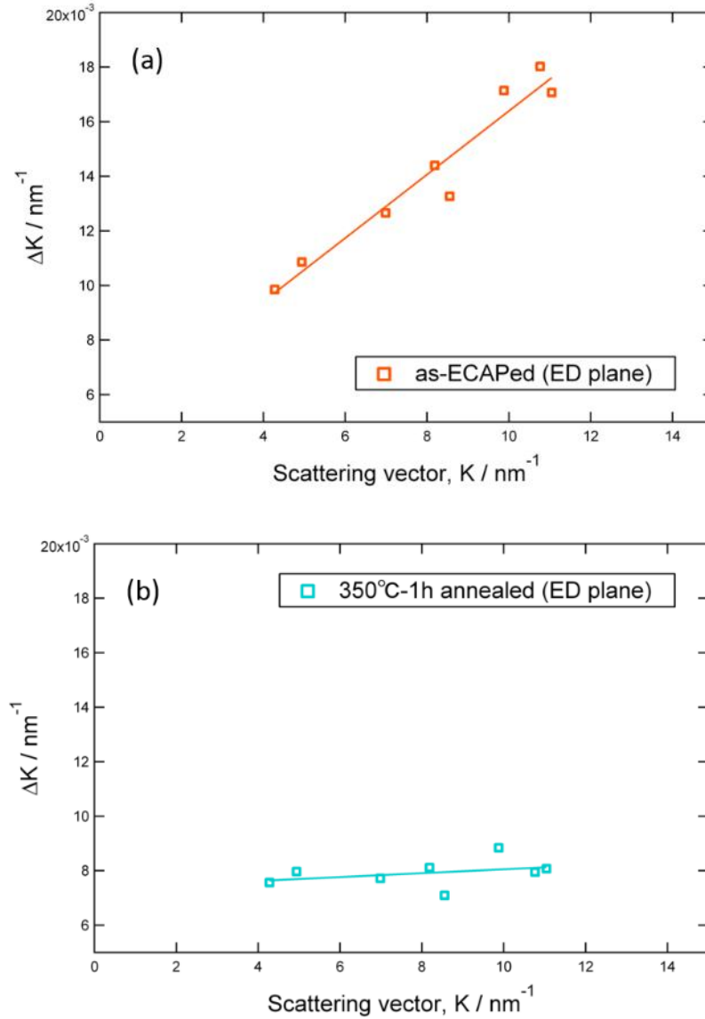
Figure 4.4 Williamson-Hall plots for two specimens (the as-ECAP processed specimen and the ECAP processed and 350C° annealed specimen), from which the lattice strain \epsilon could be obtained by linear fitting.
