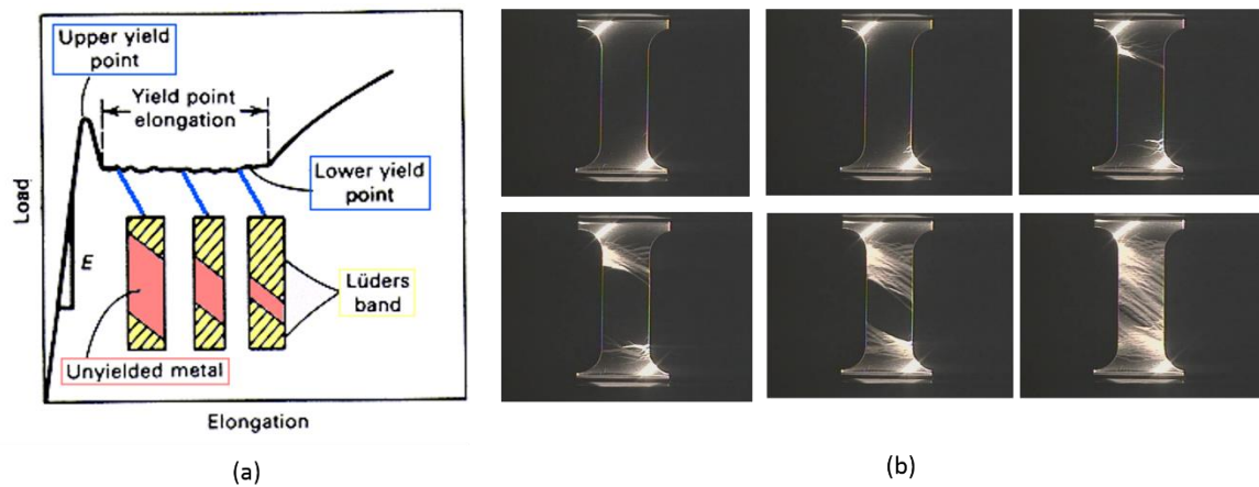
Figure 1.2 (a) An illustration of the tensile stress-strain curve exhibiting yield drop and propagation of Lüders band, and [1] (b) The Lüders band propagation during a tensile test in a low carbon steel, captured by a camera [2].
