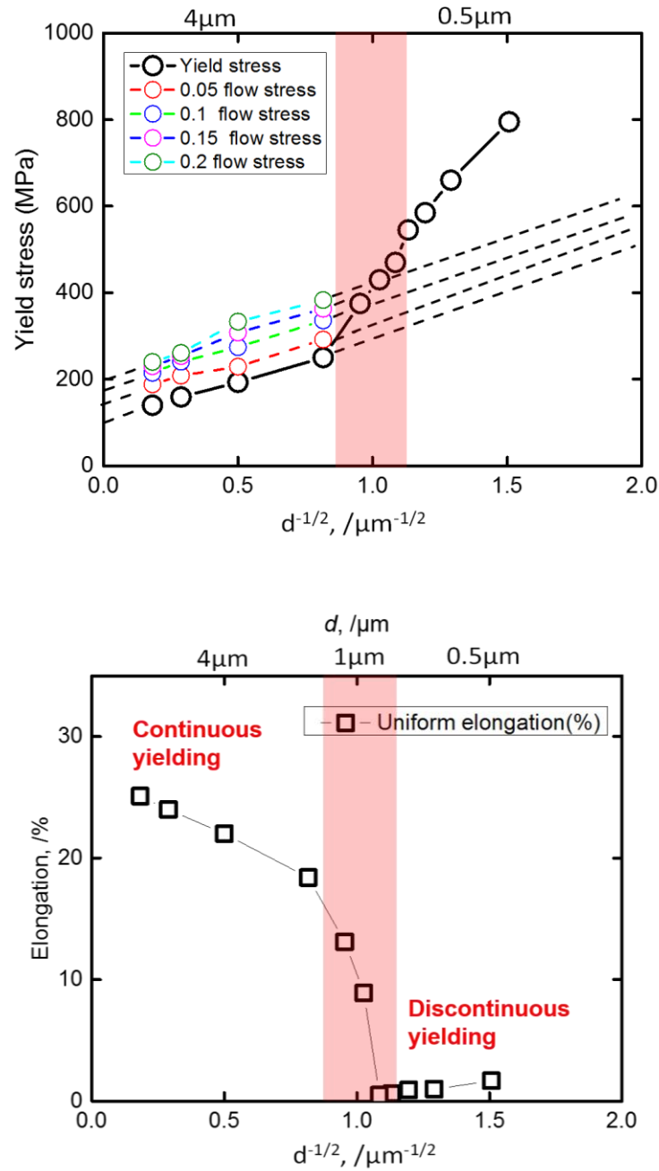
Figure 3.7 Yield stress, flow stresses at different true strains of 0.05, 0.1, 0.15, and 0.2 and the uniform elongation plotted against the inverse square root of the mean grain size. The region colored in red is the range where the yield stress overtakes the flow stress and the dramatic drop in the uniform elongation occurs.
