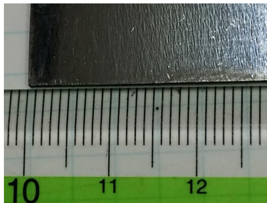
Figure 3.13 Surface morphology of the ARB processed and 540°C annealed specimen with a grain size d=0.8\ \mu\text{m} after 5% post-annealing cold rolling.
