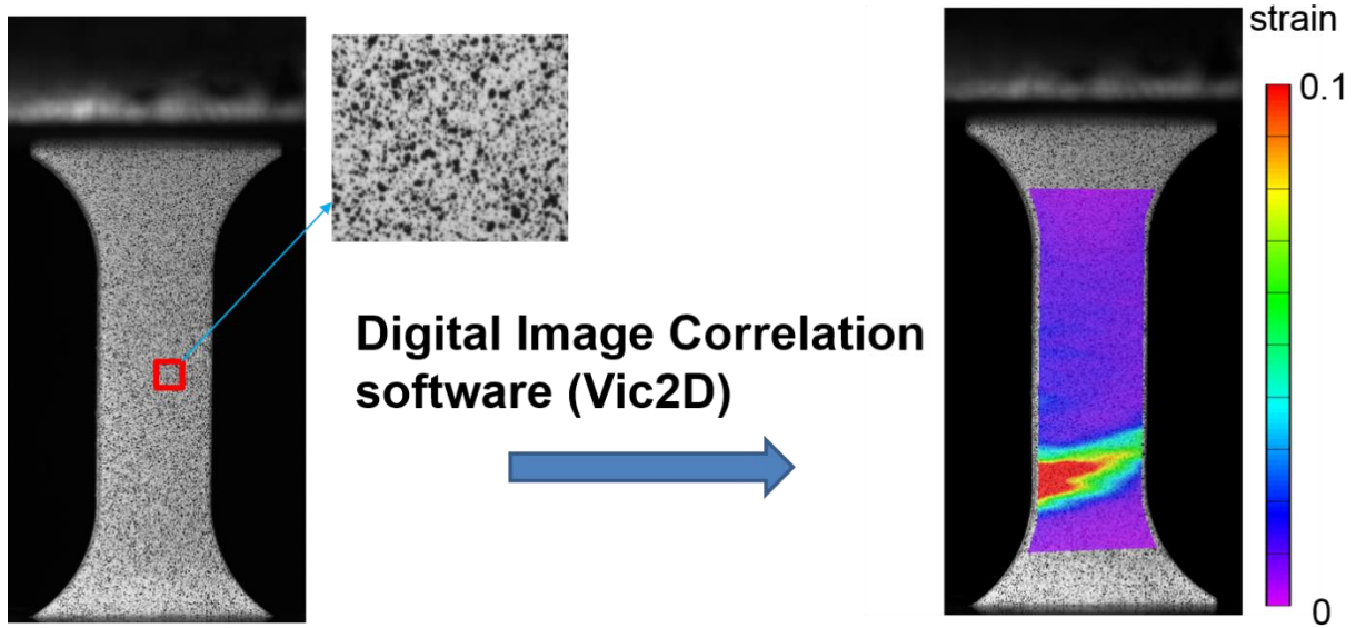
Figure 3.8 A digital image taken by the CCD camera during a tensile test (left hand side) and the strain contour calculated by the DIC software (right hand side).
