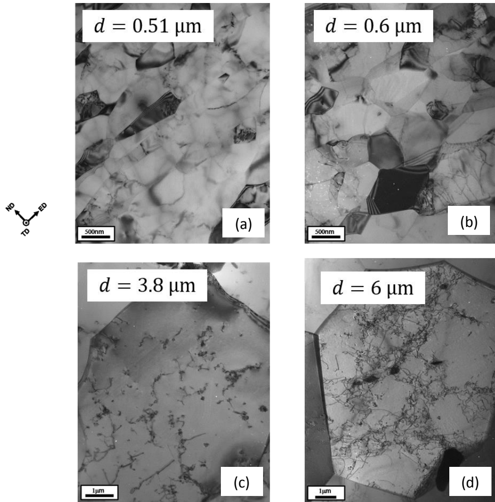
Figure 4.18. Microstructures of the specimen having grain size (a) d=0.51 \mu\text{m} (b) d=0.6 \mu\text{m} (c) d=3.8 \mu\text{m} (d) d=6 \mu\text{m} , observed by TEM.
