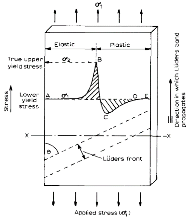
Figure 1.5 Schematic illustration of the transverse stress distribution across the Lüders band [11].
