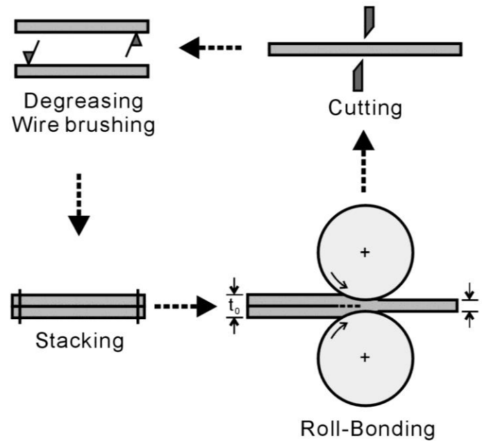
Figure 3.1 Illustration of the accumulative roll-bonding (ARB) process.
