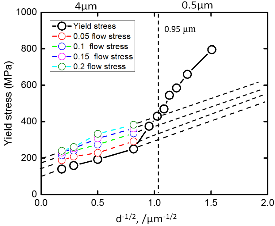
Figure 3.6 Flow stresses at different true strains of 0.05, 0.1, 0.15, and 0.2 plotted against the inverse square root of the mean grain size. The Hall-Petch slopes for the flow stresses at given strains show similar values of around 250 \text{ MPa} \cdot \mu\text{m}^{1/2} .
