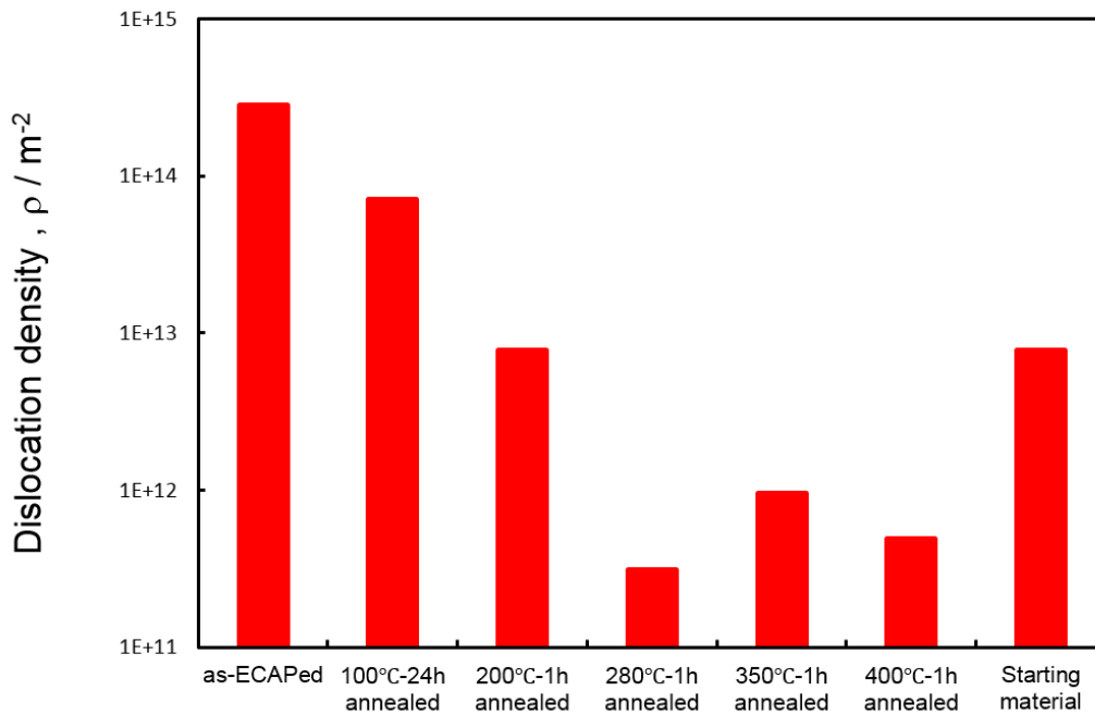
Figure 4.5 The dislocation densities of the as-ECAP processed specimens and the ECAP processed and annealed specimens measured by XRD.
