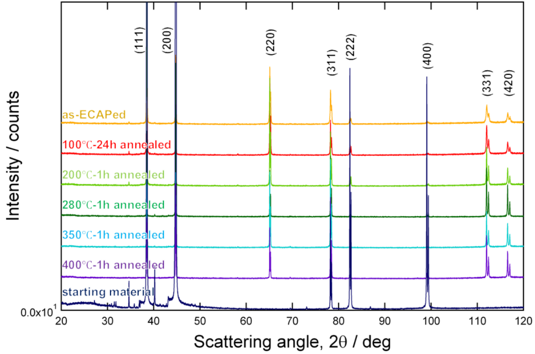
Figure 4.3. Diffraction patterns of the starting material as well as the as-ECAP processed and subsequently annealed specimens.
