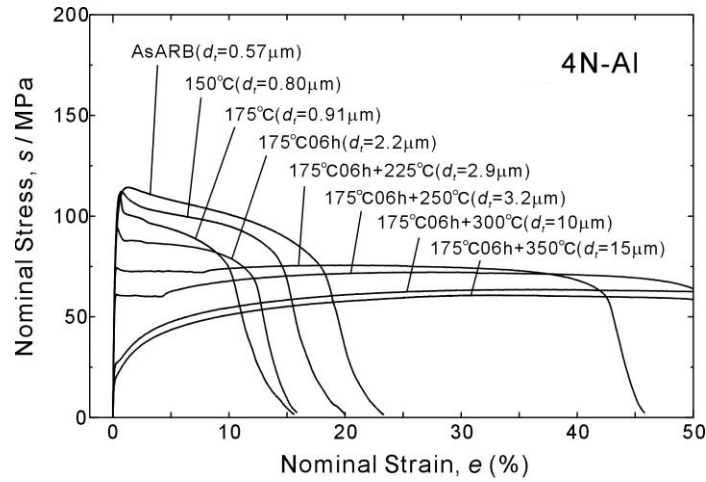
Figure 1.7 Stress-strain curves of the 4N-Al having different grain sizes, fabricated by the ARB and subsequent annealing processes [17].
