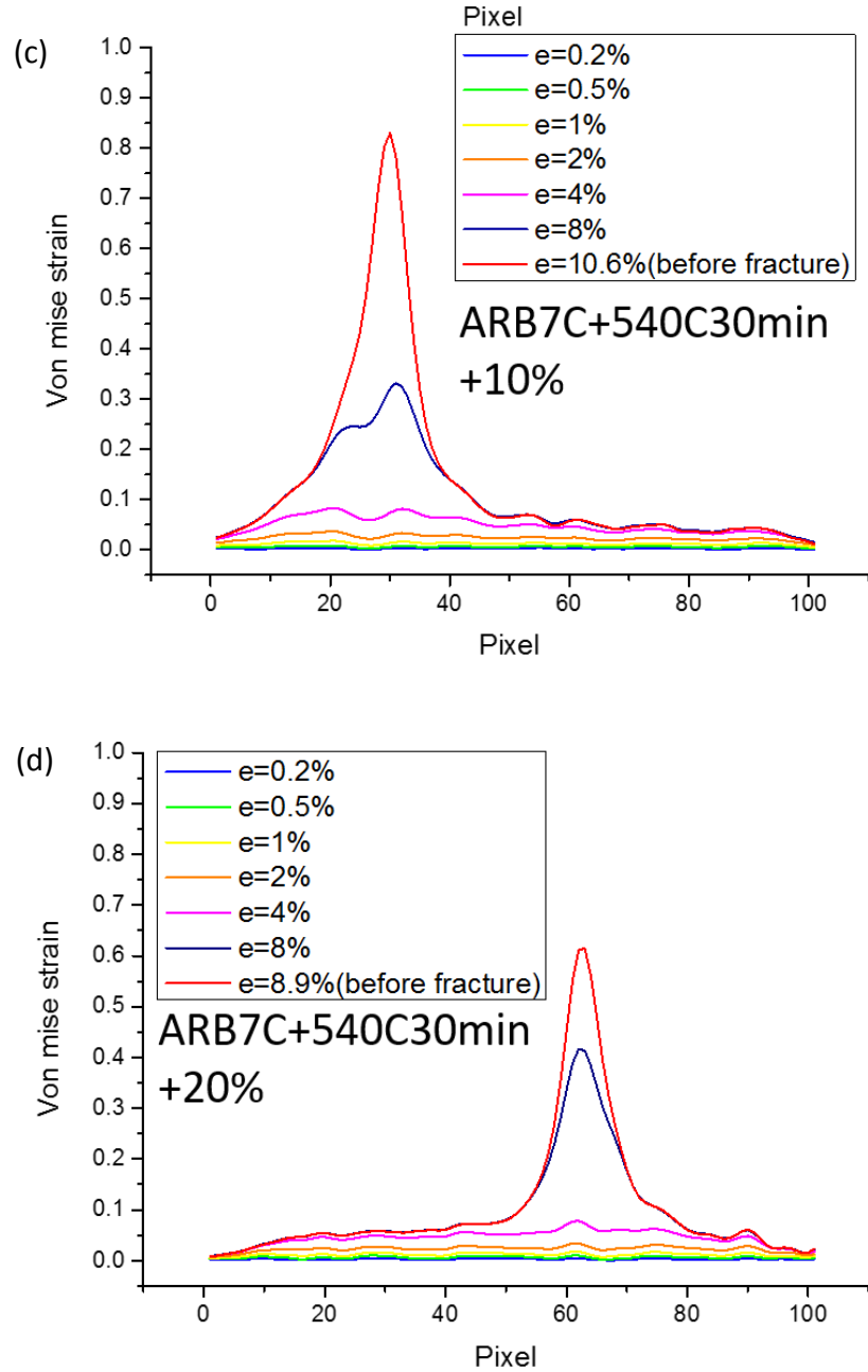
Figure 3.21 (Continued) Strain distribution maps of the specimen having d=0.8 \mu\text{m} and cold-rolled by (a) 0% (b) 5%, (c) 10% and (d) 20%.
