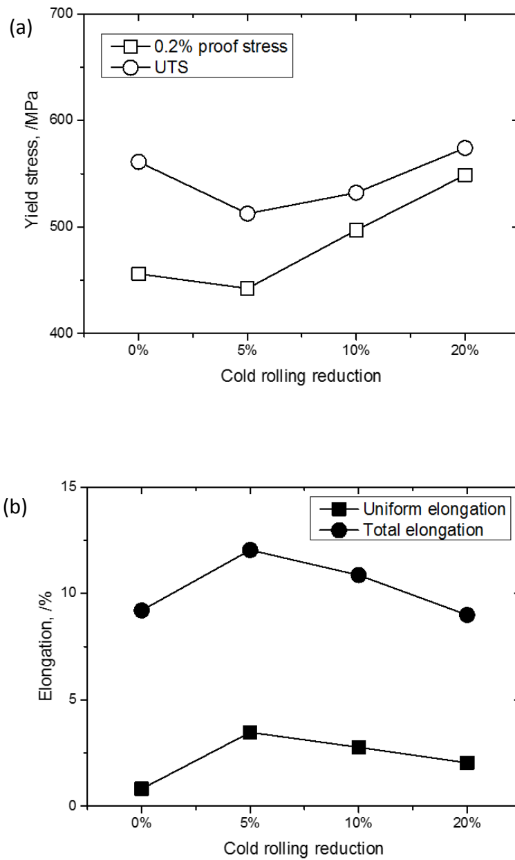
Figure 3.20 The yield stress and UTS (a), uniform elongation and total elongation (b) of the specimen having d=0.8 \mu\text{m} are plotted as the function of the cold rolling reduction.
