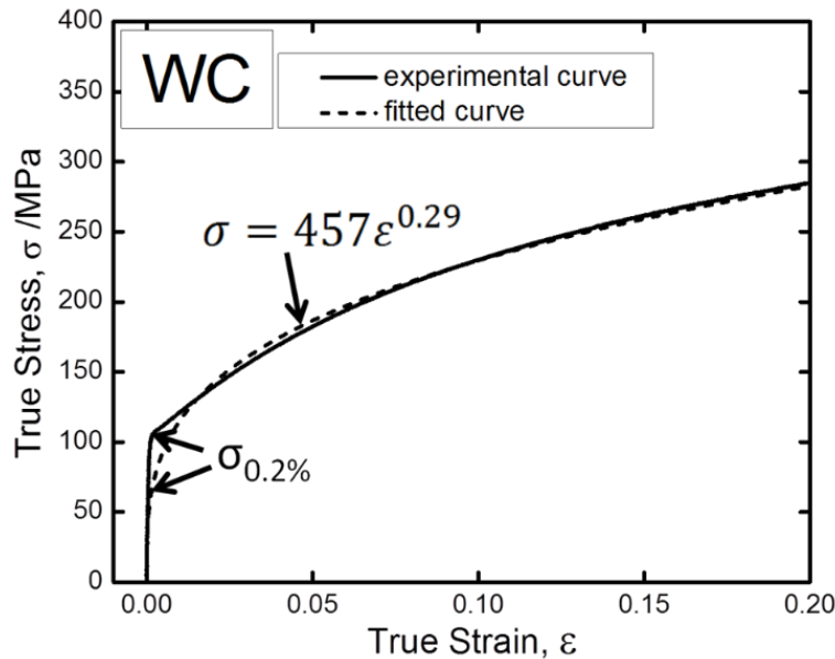
Figure 2.14 The extrapolation process on a WC specimen is shown. Note that the yielding behavior of the WC specimen is somewhat discontinuous compared with the extrapolated curve.
