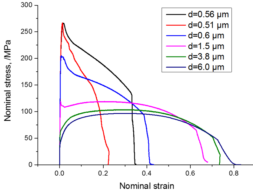
Figure 4.9 Monotonic tensile stress-strain curves of the as-ECAP processed specimen ( d=0.56\ \mu\text{m} ) and subsequently annealed specimens having different mean grain sizes ranging from 0.56\ \mu\text{m} to 6\ \mu\text{m} .
