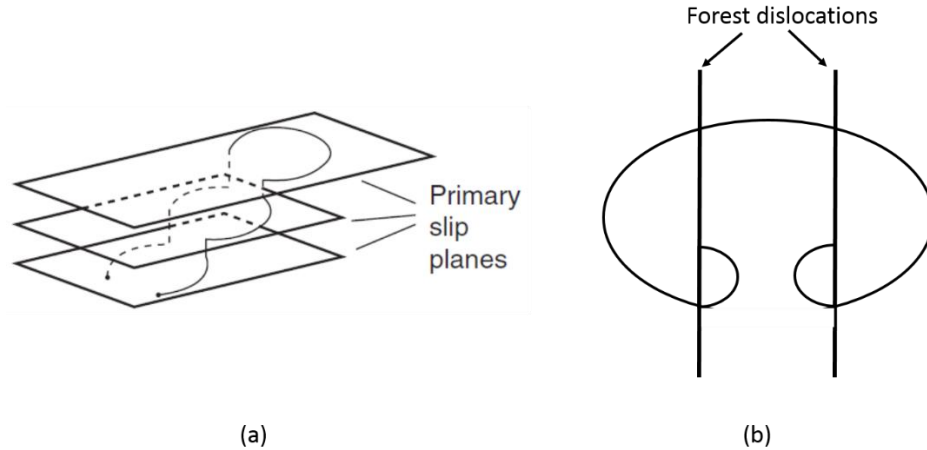
Figure 1.9 Illustration of the dislocation multiplication by (a) double cross-slip and (b) dislocation segment acting as a Frank-Read source.
