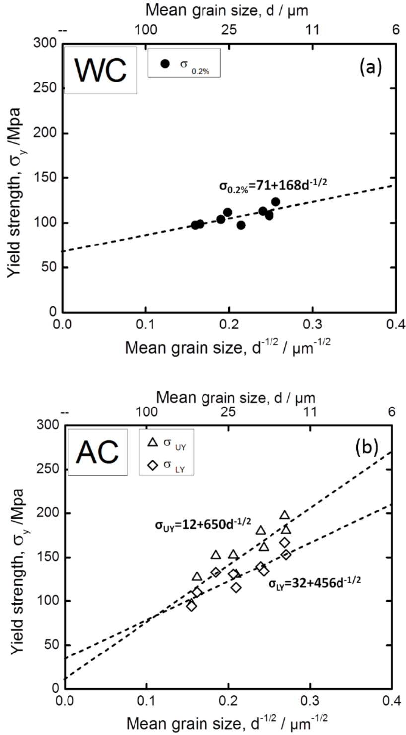
Figure 2.8 Hall-Petch relationships for the WC specimens (a) and for the AC specimens (b).
