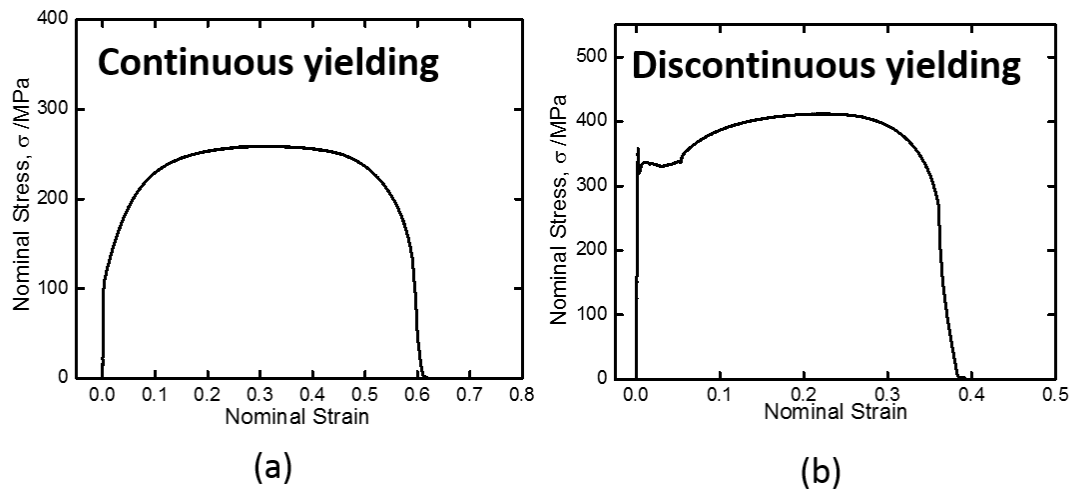
Figure 1.1 Illustrations of the tensile stress-strain curves exhibiting (a) continuous yielding and (b) discontinuous yielding.
