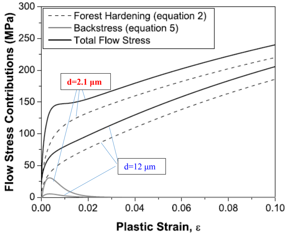
Figure 1.11 Evolution of the back stress, forest hardening and total flow stress of the copper with d=2.1 \mu\text{m} and d=12 \mu\text{m} , calculated by Sinclair's model [30].
