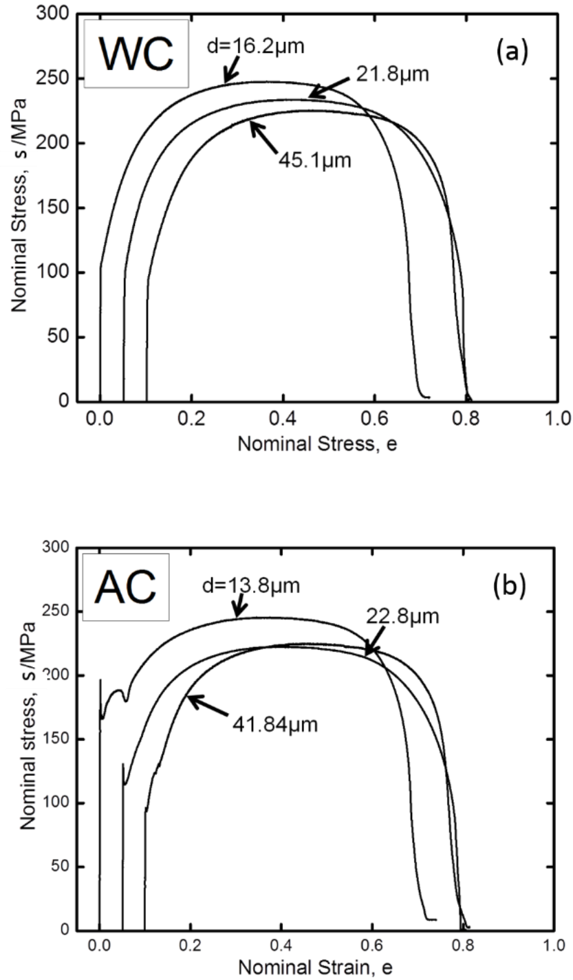
Figure 2.3 Selected nominal stress-strain curves of the water-cooled (WC) (a) and the air-cooled (AC) (b) specimens with different grain sizes.
