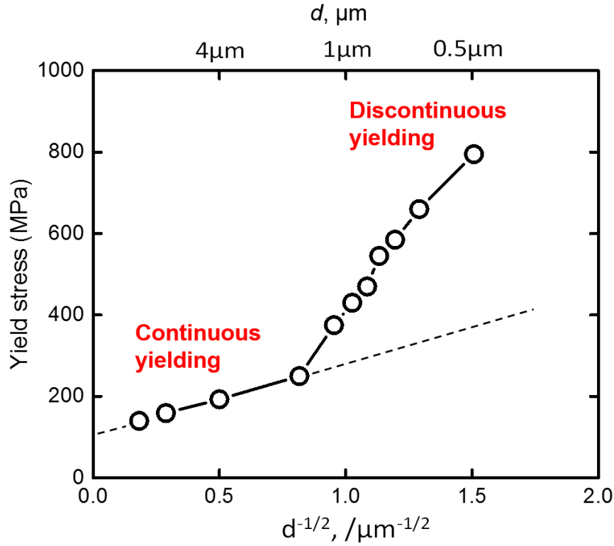
Figure 3.4 Yield stress of the IF steel specimens plotted as a function of inverse square root of the mean grain size (Hall-Petch plot).
