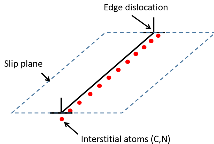
Figure 1.3 Illustration of interstitial solute atoms segregating on an edge dislocation lying on the slip plane in a low carbon steel.
