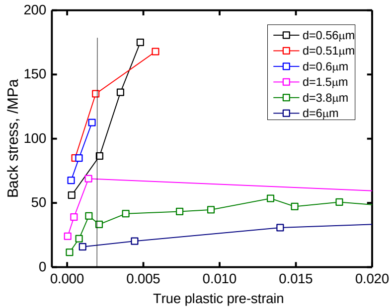
Figure 4.16 Experimentally obtained back stresses at small plastic pre-strain region (0-0.02). The back stresses at the pre-strain of 0.002 of the specimens can be estimated from this figure.
