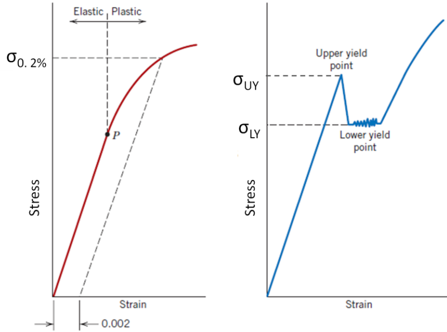
Figure 2.7 The different determination of the yield strength for (a) continuous yielding and (b) discontinuous yielding [8].
