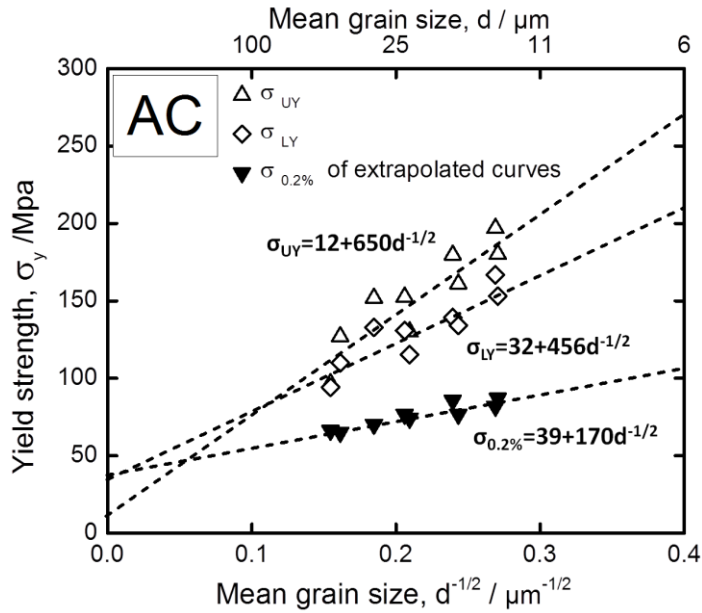
Figure 2.13 The \sigma_{UY} , \sigma_{LY} and \sigma_{0.2\%} measured from the stress-strain curves of the AC specimens were plotted against d^{-1/2} . The Hall-Petch relationship of each kind of yield stress is also given.
