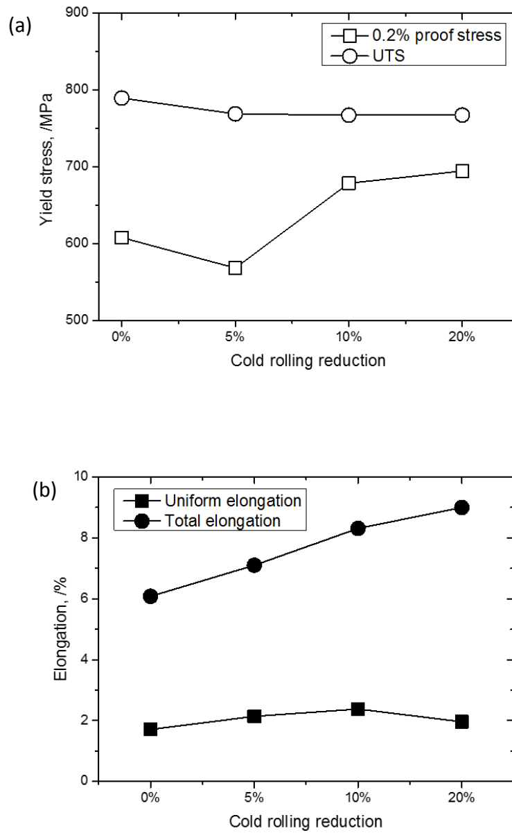
Figure 3.17 The yield stress and UTS (a), uniform elongation and total elongation (b) are plotted as the function of the cold rolling reduction of the as-ARB processed specimen and ARB processed and cold-rolled specimen.
