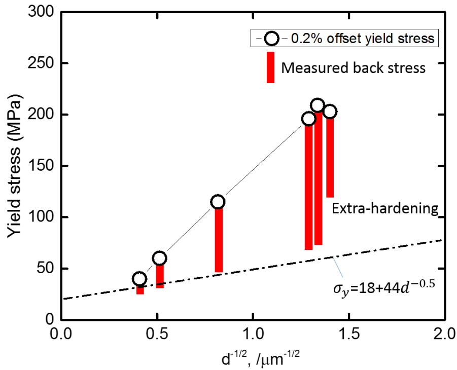
Figure 4.17. The back stresses at 0.2% pre-strain estimated from Figure 4.15 are indicated as the red bars in the Hall-Petch plot. The 0.2% proof stress obtained from the monotonic tensile test for the specimens are also plotted. The Hall-Petch relationship obtained in the conventionally coarse grain sized specimens is also given.
