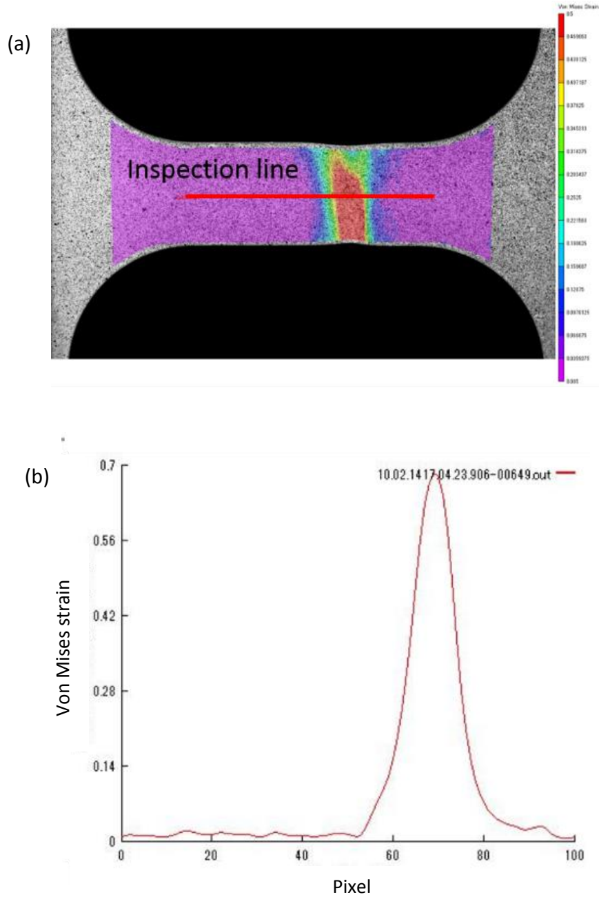
Figure 3.9 (a) A strain contour map obtained from the DIC analysis, and (b) equivalent strain distribution along the inspection line on the gauge part shown in (a).
