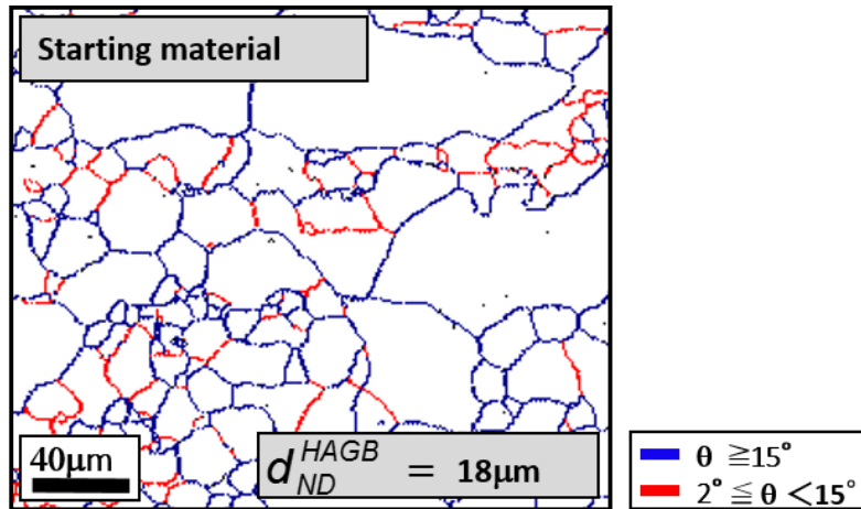
Figure 4.1 EBSD grain boundary map showing the microstructure of the starting material of 1100-Al.
