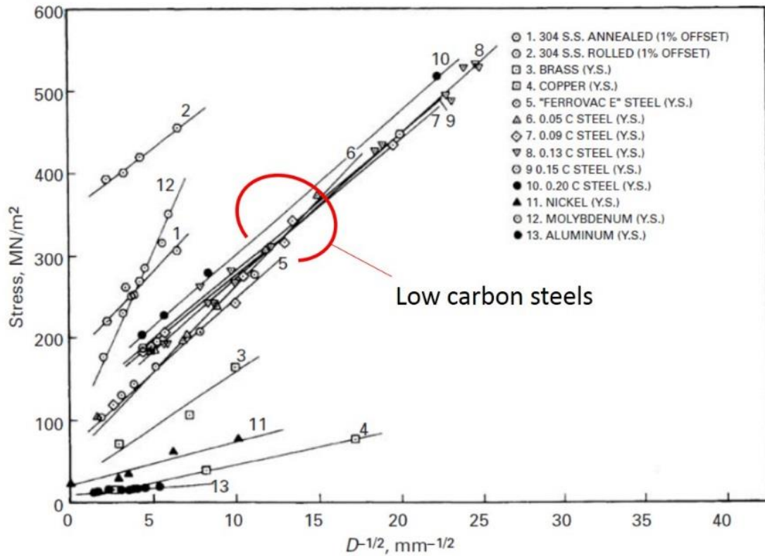
Figure 2.1 The Hall-Petch relationships for several common engineering materials [4].
