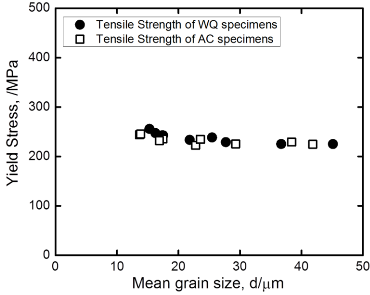
Figure 2.6 Tensile strength as a function of the mean grain size for the water-cooled and the air-cooled specimens.
