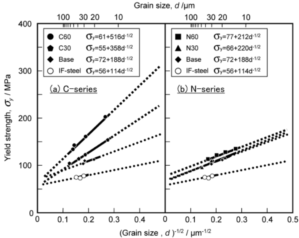
Figure 2.10 Hall-Petch slope, k_y , decreased with the decrease of carbon (left hand side) and nitrogen content (right hand side) [15].
