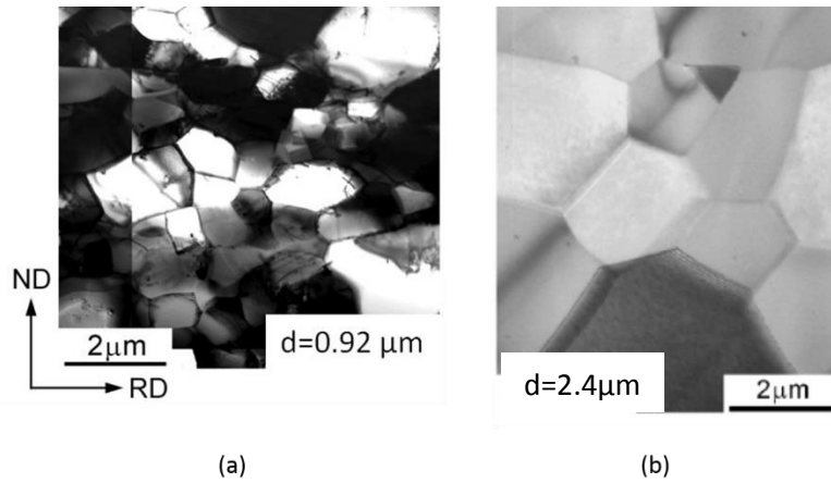
Figure 1.8 TEM micrographs showing the “clean” microstructures in the (a) IF steel [26] and (b) 4N-Al [17] having fine grain sizes, fabricated by ARB and subsequent annealing process. The mean grain sizes are indicated in the figure.
