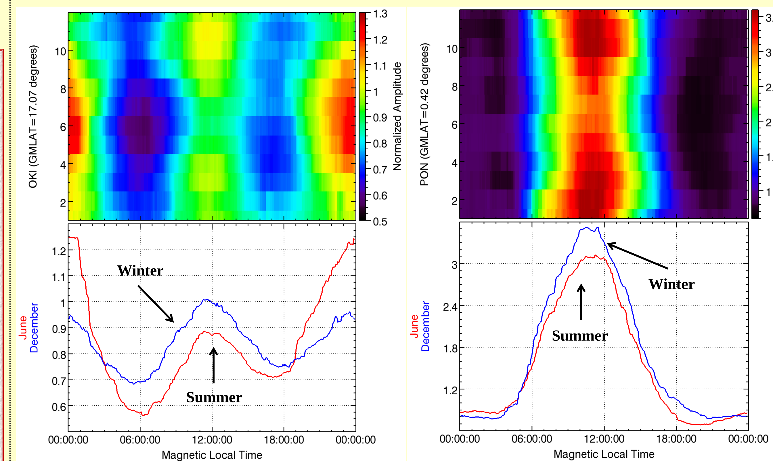
Fig. 5. Seasonal variation of SC amplitude from the subauroral region (1) to the magnetic equator (4). In the subauroral and middle latitudes, the SC amplitude tends to enhanced significantly, while it tends to depress slightly in a region from the low latitude to equator. The seasonal dependence indicates a different feature between the middle latitude and magnetic equator.
