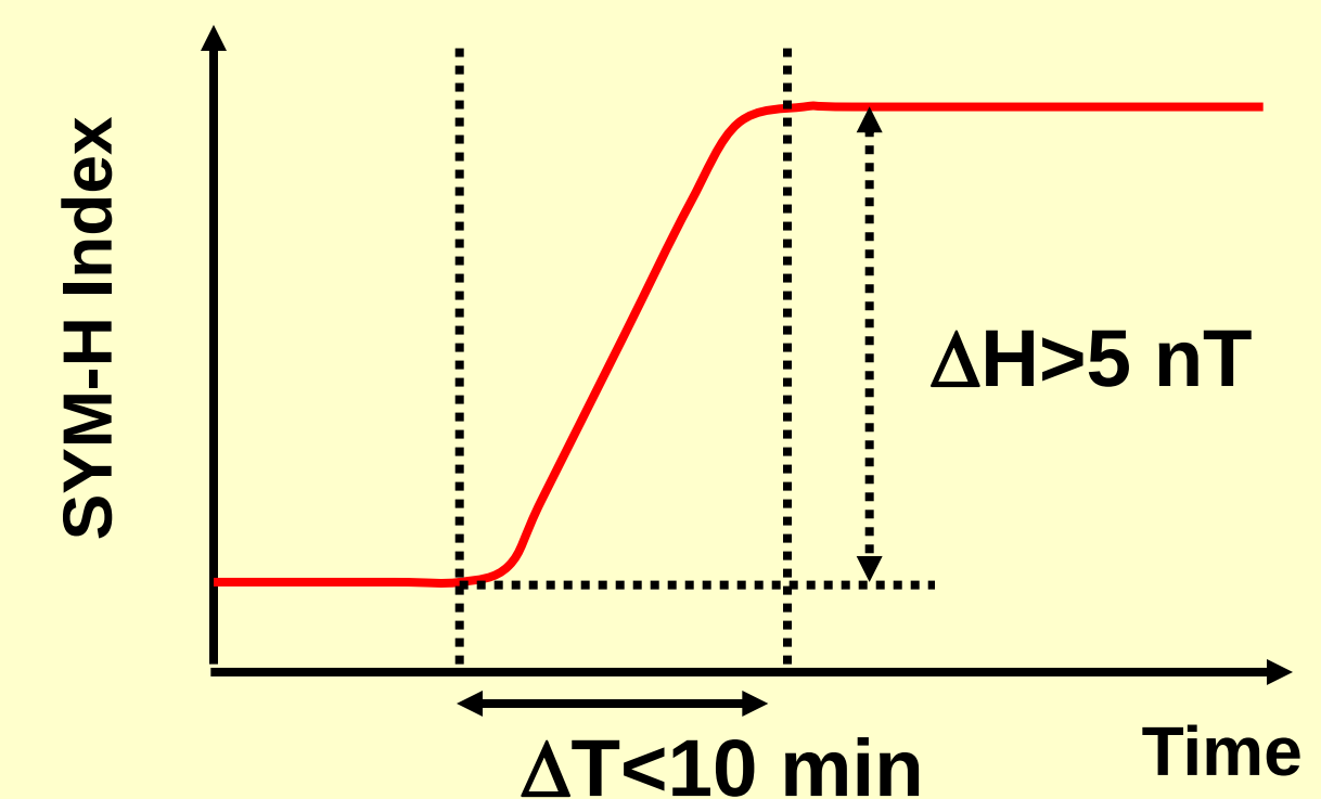
Fig. 2. An schematic view of the SYM-H variation associated with an abrupt increase of solar wind dynamic pressure.
