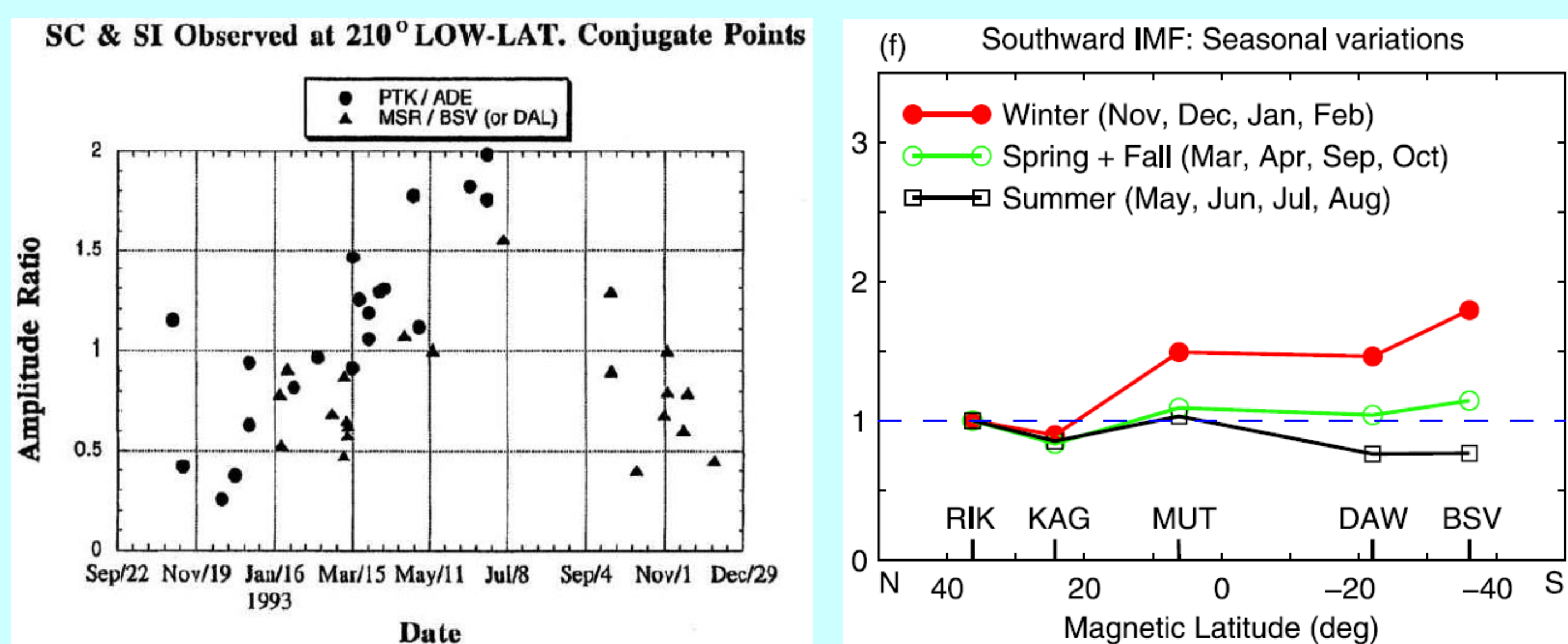
Fig.1. Seasonal variation of north-south asymmetry of SC amplitude in the middle latitudes as a function of day and month (a) [Yumoto et al., 1996] and in a region from the middle latitudes to magnetic equator as a function of magnetic latitude (b) [Huang and Yumoto, 2006].
