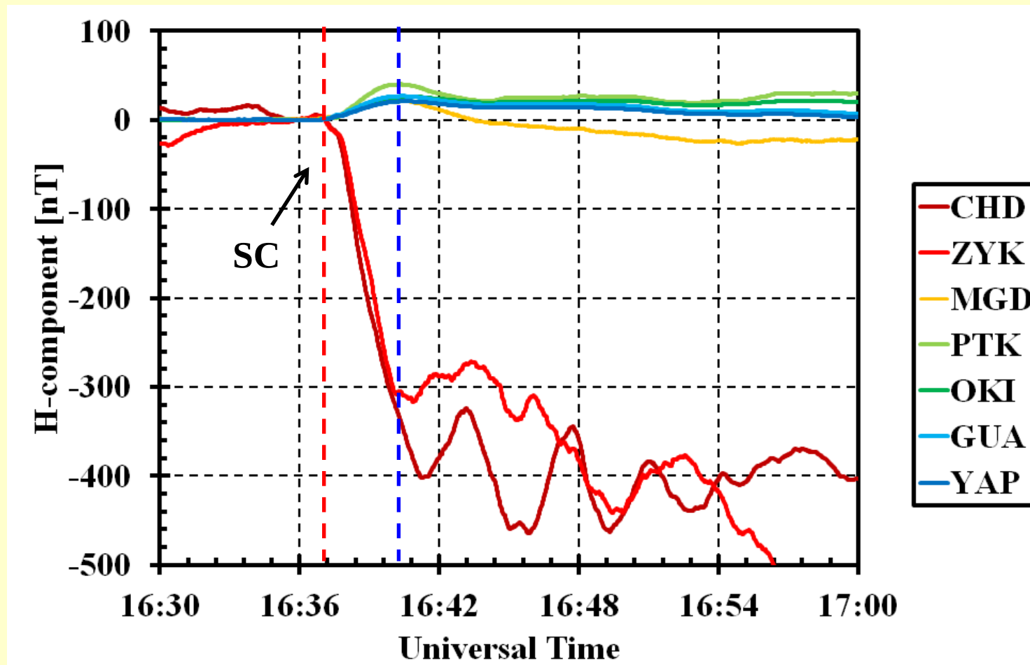
Fig. 3. An SC event at 16:35:48 (UT) on September 7, 2002 observed at 7 stations (CHD, ZYK, MGD, PTK, OKI, GUA, and YAP). The vertical dotted red and blue lines indicate the SC onset and the maximum of SC amplitude in the low latitude (OKI).
