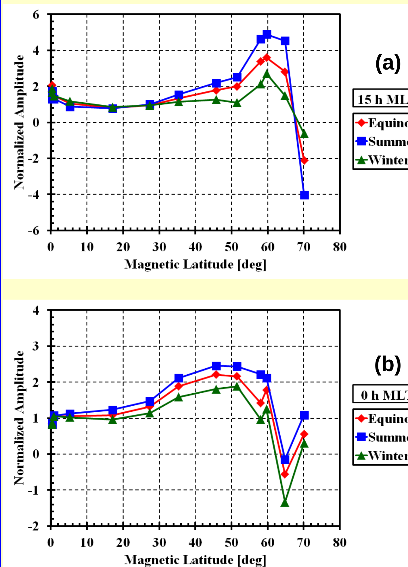
Fig. 6. Latitudinal profiles of SC amplitude in a wide region from high latitudes (GMLAT=70.08°) to magnetic equator (GMLAT=0.42°) of the afternoon (15 h MLT) (a) and midnight (0 h MLT) (b) sectors, respectively. The red, blue and green lines are SC amplitudes in three periods of equinox (2-4 and 8-10), summer (5-7) and winter (11-1).
