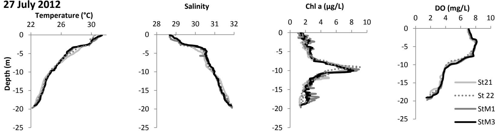
Figure 3-14: Vertical profiles of temperature, salinity, chlorophyll a ( \mu\text{g L}^{-1} ) and dissolved oxygen ( \text{mg L}^{-1} ) at Sts. 21, 22, M1 and M3 in June and July in 2012.
