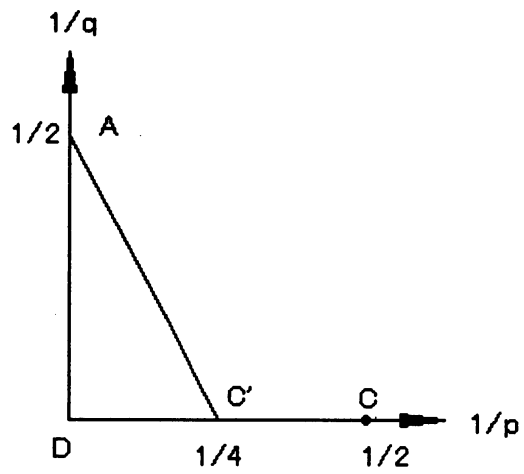
FIGURE 2. The case n = 3 .
