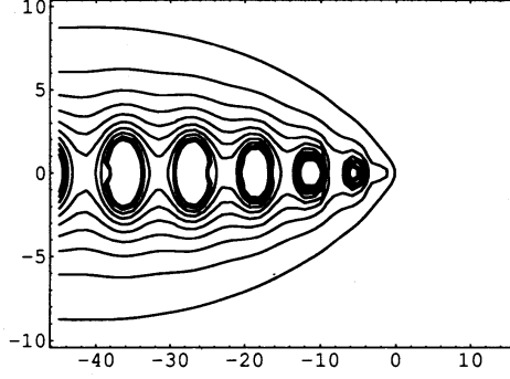
Figure 1: the contourplot for M = 3 , |e^{E/7} T_2^{(1)}(E)|
