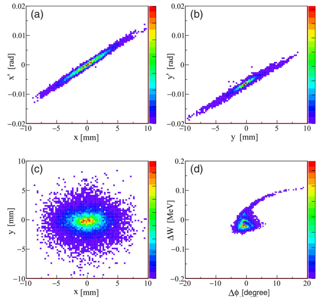
FIG. 8. Calculated phase space distributions at IH exit. (a) the horizontal divergence angle x' vs x , (b) the vertical divergence angle y' vs y , (c) y vs x , and (d) \Delta W (W = 4.5 \text{ MeV}) vs \Delta\phi .
