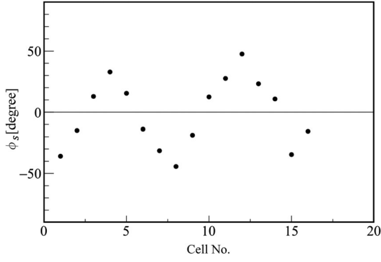
FIG. 3. Optimized phase ( \phi_s ) array results as function of cell (gap) number.
