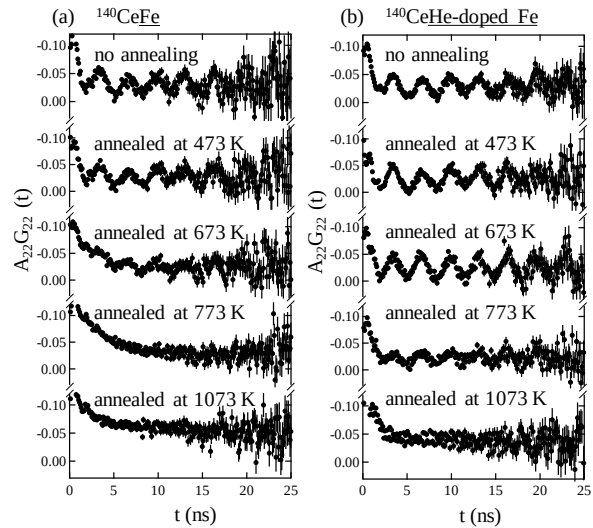
Fig. 1. Room-temperature TDPAC spectra for (a) ^{140}\text{CeFe} and (b) ^{140}\text{CeHe-doped Fe} , subjected to no annealing, 0.5-h annealing in vacuum at 473, 673, 773 and 1073 K (after annealed at 873 and 973 K).
